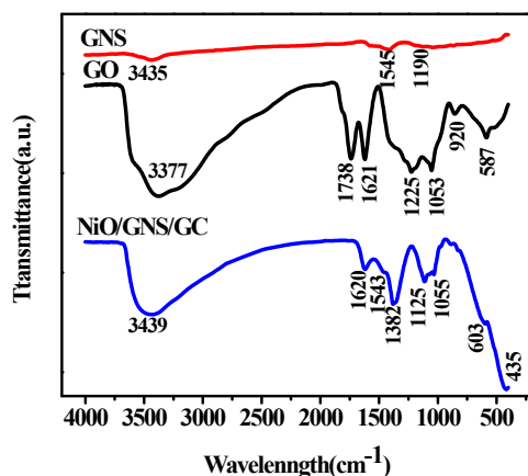
Fig.S1.FT-IR spectra of GNS, GO and NiO/GNS/GC.
