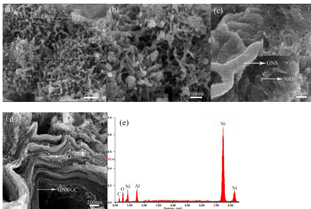
Fig.S2. SEM images of (a) pure NiO, (b) higher magnification of pure NiO (higher magnifications of the (a) square frame regions), (c) NiO/GNS composites (inset higher magnifications of the square frame regions), (d) NiO/GNS/GC composites, (e) EDX pattern of the NiO/GNS/GC.
