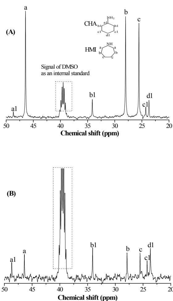
Fig. S1. ^{13}\text{C} NMR spectra of the mother liquor: (A) SB-1-L and (B) SC-1-L.
