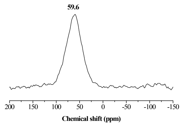
Fig. S2. ^{27}\text{Al} NMR spectra of SF-1-L.
