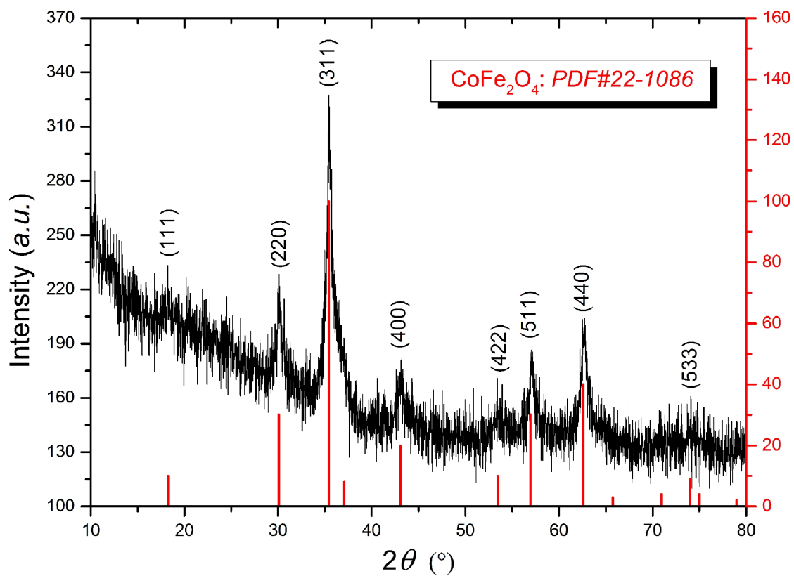
Fig. S1. Representative XRD pattern of the nanoparticle sample obtained by calcining at 400°C for 5 h with the CHR of 7°C/min.
