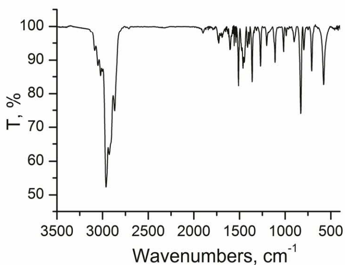
Figure 1: FTIR spectra of nanocapsule 2.
