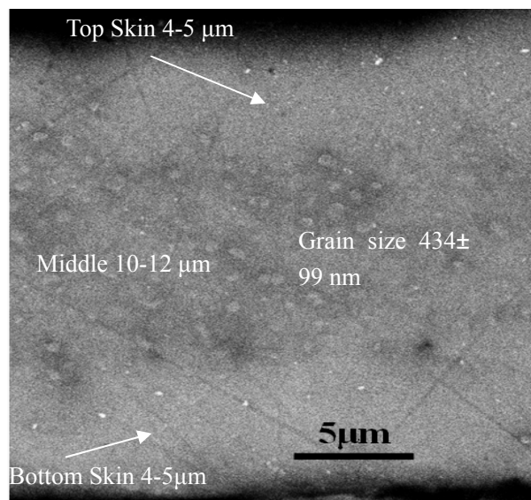
Figure S1 The secondary electron SEM image for the cross-section of the ribbon annealed under the transverse field
