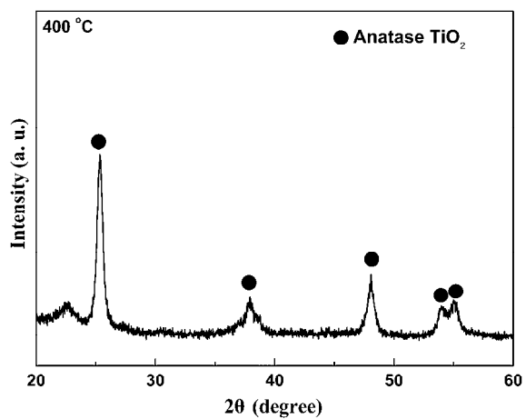
Fig. S1. XRD pattern of the TiO 2 nanofibers calcined at 400°C for 2 h in air atmosphere.
