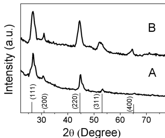
Figure S1. XRD patterns of as-synthesized Cu 2-x Se nanoplates with (A) and without (B) the precipitation of Sn-X complex.
