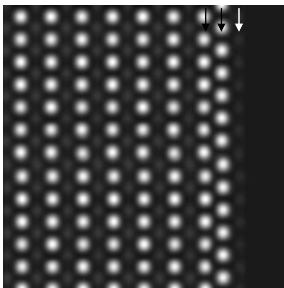
Fig. S2. HAADF multi-slice simulation of Pt 3 Fe with a Fe only outer layer (indicated by the white arrow) followed by two layers of Pt only layers (indicated by the black arrows).
