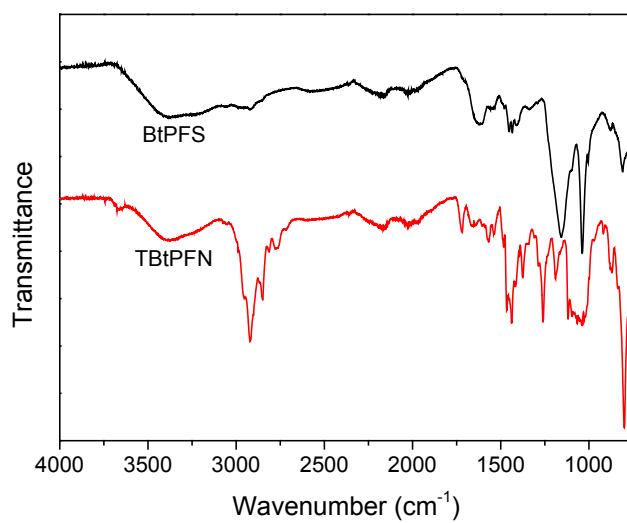
Fig. S1 FT-IR spectra of BtPFS and TBtPFN.
