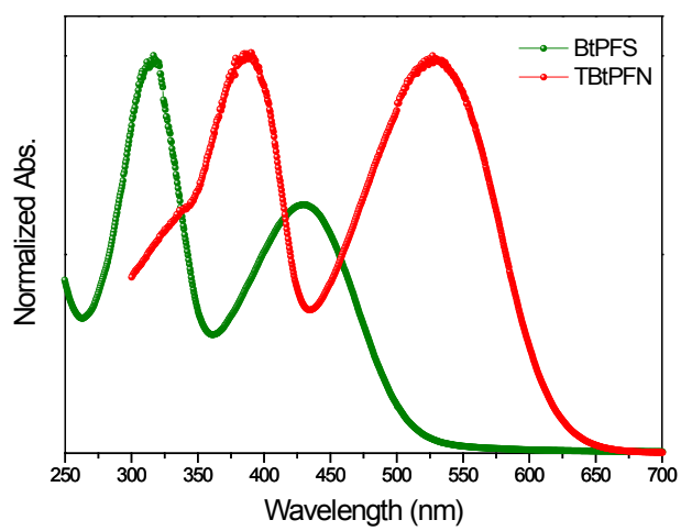
Fig. S2 UV spectra of BtPFS and TBtPFN.
