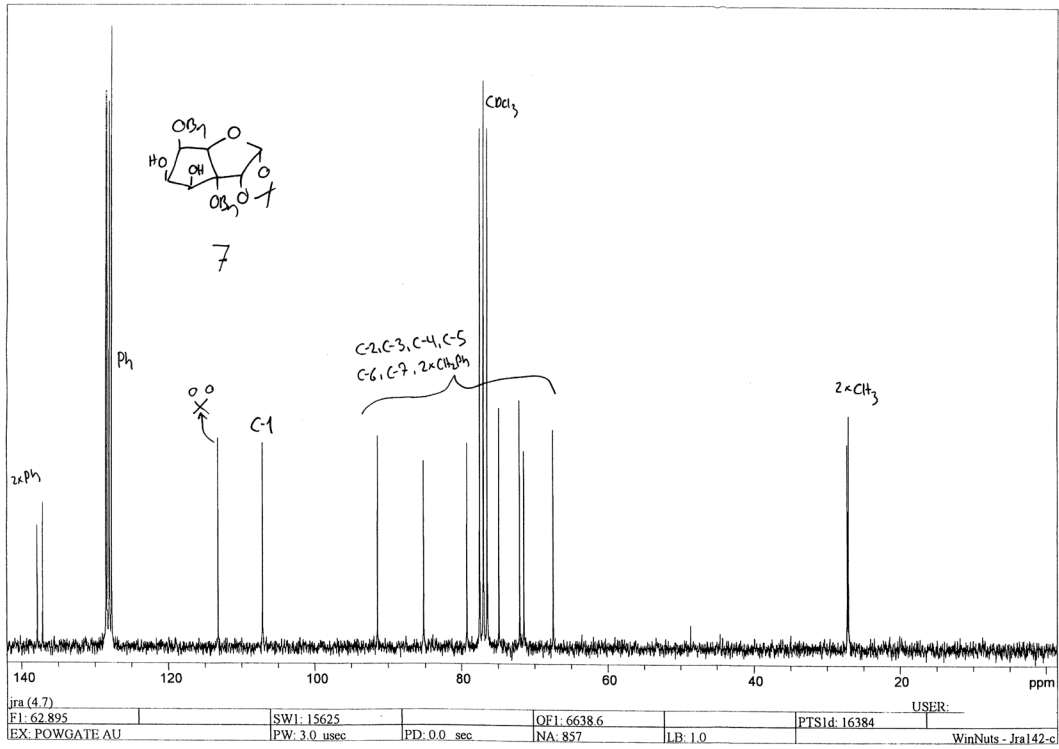
13 C NMR spectrum of compound 7
