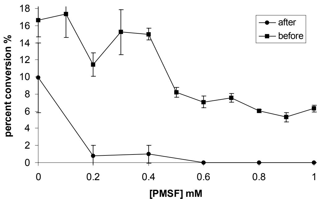
Graph depicting % conversion of the \gamma -lactam substrate in the presence of varying concentrations of PMSF before and after catalytic turnover.
