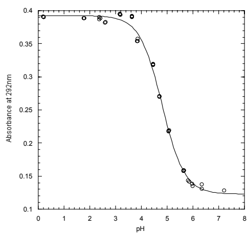
Supplementary Figure 2: pH Titration plots for compounds 5 (upper left), 6 (upper right), 7 (lower left) and 2-amino-4-methoxy-7-methyl-7 H -pyrrolo[2,3- d ]pyrimidine ( 18 ) (lower right).
