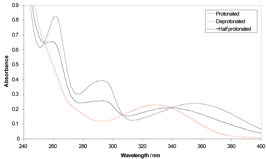
Supplementary Figure 1: Absorption spectra at neutral and acidic pH for compounds 5 (upper left), 6 (upper right), 7 (lower left) and 2-amino-4-methoxy-7-methyl-7H-pyrrolo[2,3-d]pyrimidine ( 18 ) (lower right).
