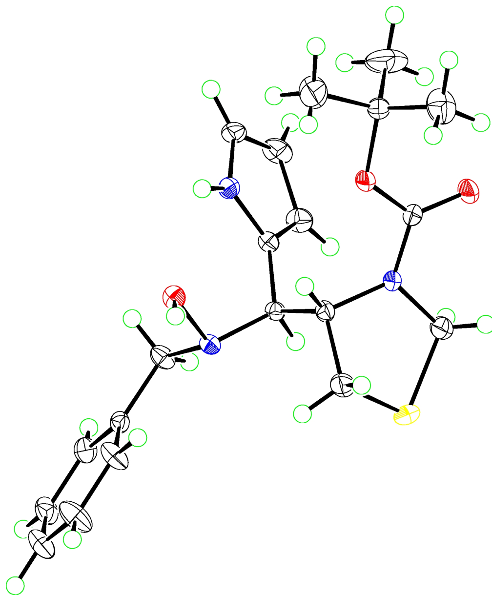
X-ray Diagram for 7a
