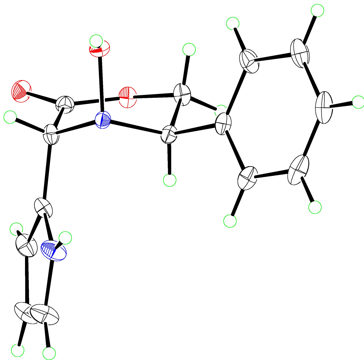
X-ray Diagram for 11
