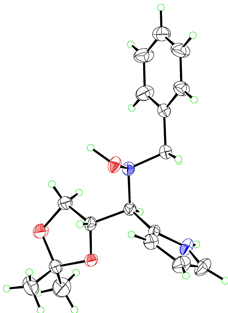
X-ray Diagram for 7b
