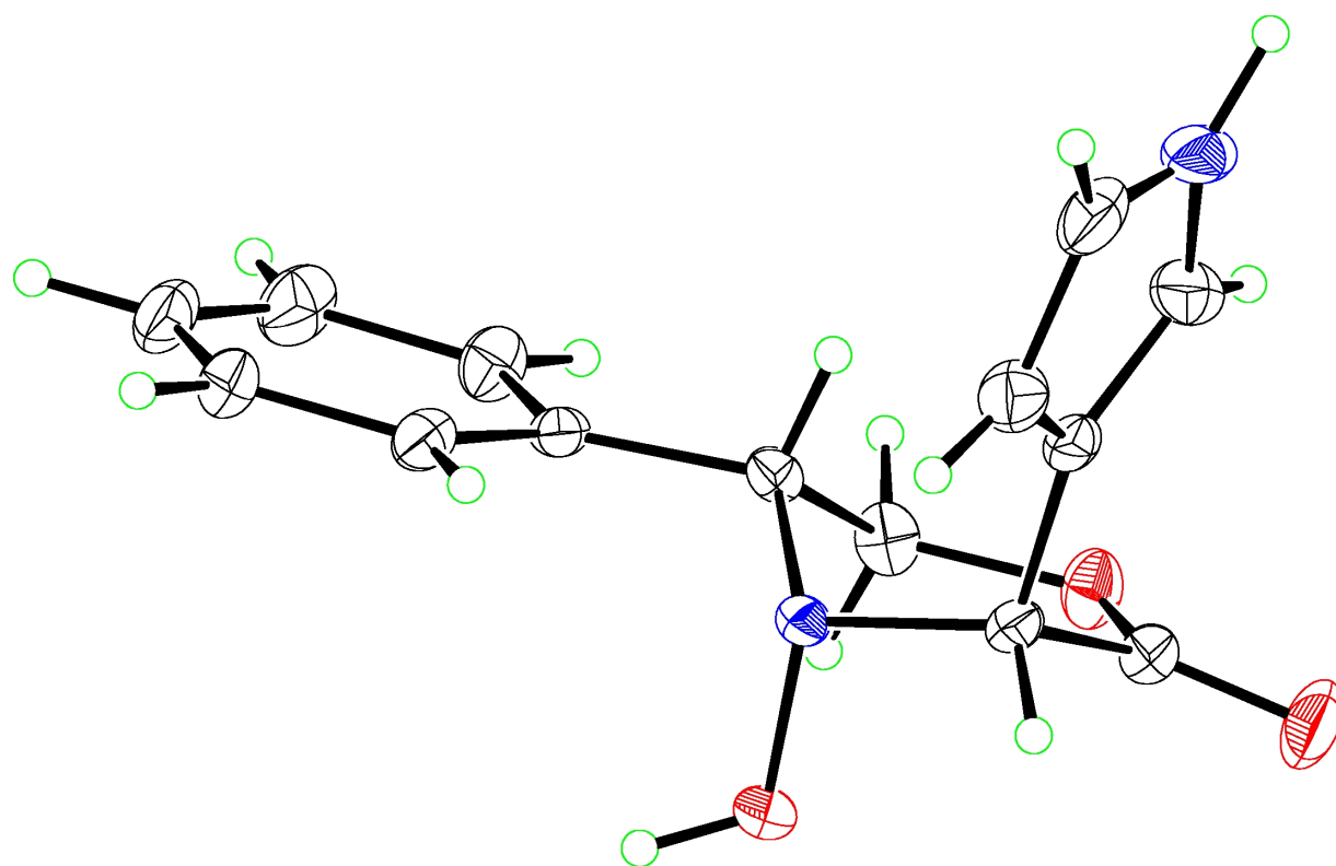
X-ray Diagram for 17
