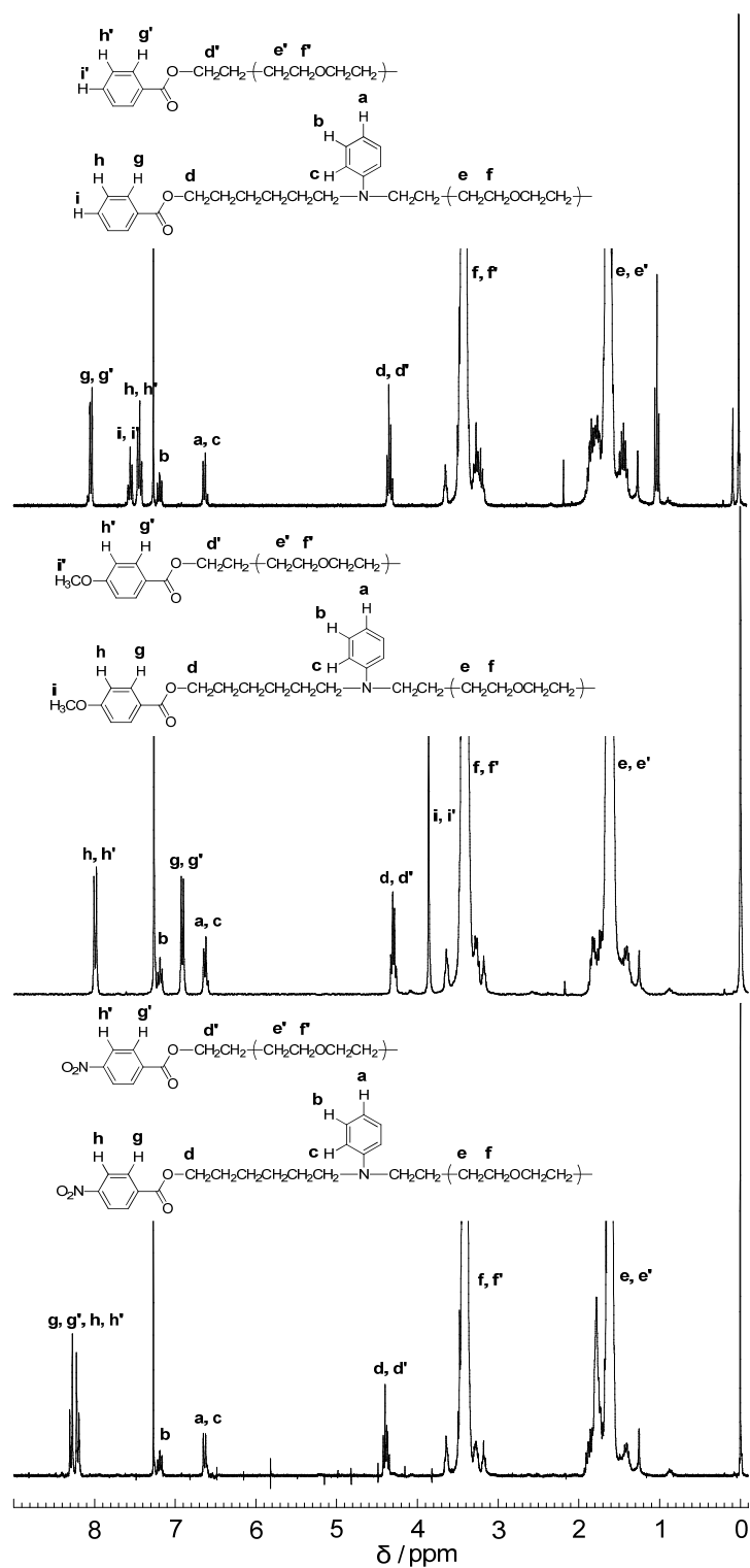
Figure S2. ^1\text{H} NMR spectra (300 MHz) of the reaction products of poly(THF) having N -phenylazepanium salt end groups ( 2 ) with (top) benzoate, (middle) p -methoxybenzoate, and (bottom) p -nitrobenzoate benzoate anions. ( \text{CDCl}_3 , 25 ^\circ\text{C} )
