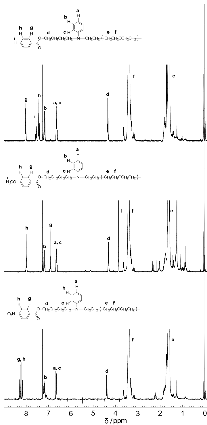
Figure S1. ^1\text{H} NMR spectra (300 MHz) of the reaction products of poly(THF) having N -phenylpyrrolidinium salt end groups ( 1 ) with (top) benzoate, (middle) p -methoxybenzoate, and (bottom) p -nitrobenzoate benzoate anions. ( \text{CDCl}_3 , 25 ^\circ\text{C} )
