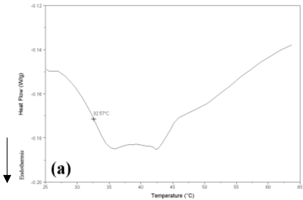
Supplementary Figure 1. DSC heating thermograms showing glass transition temperatures (+): (a) PVAc-140 ; (b) PVAc-83 .
