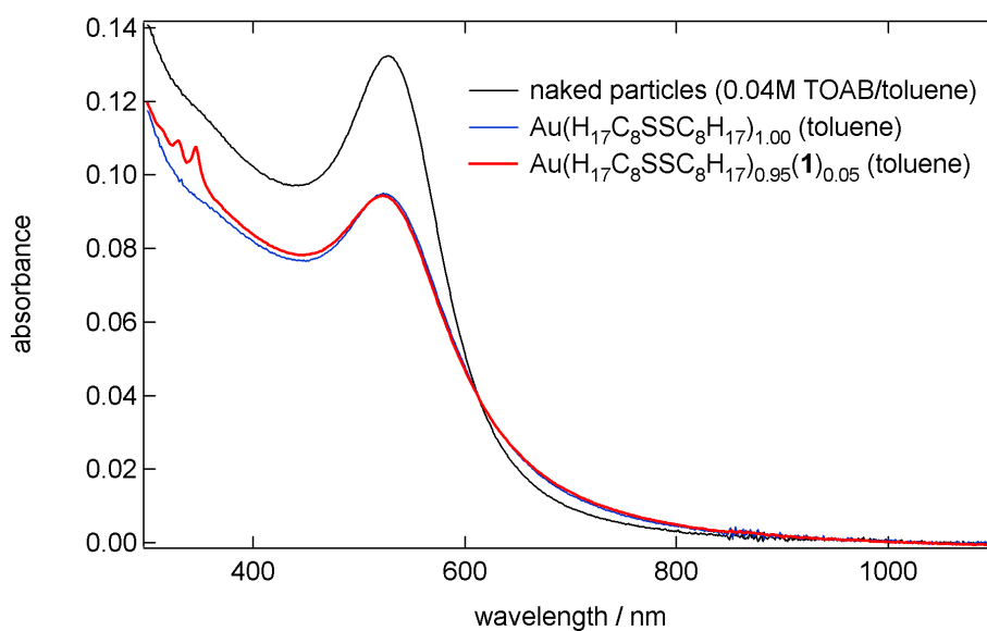
Absorption spectra of nanoparticle solutions in toluene
