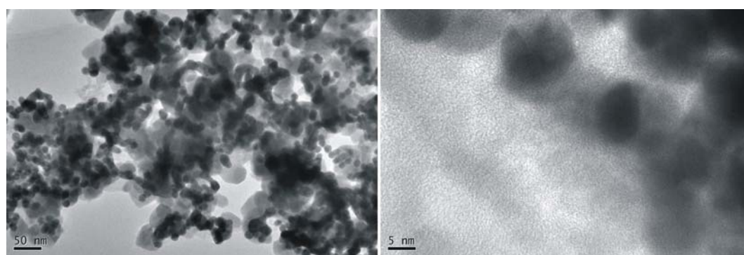
Fig S2. TEM of CuCl/Me 6 TREN with AuNPs in Water/2-propanol (1:1, volume ratio) solution. Cu(I) could be observed around AuNPs.
