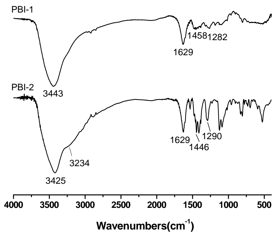
Fig. 4S FTIR spectra of PBI-1 and PBI-2 .
