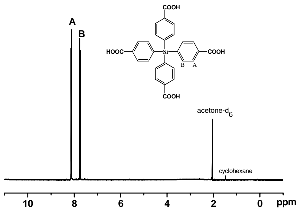
Fig. 3S ^1\text{H} NMR spectrum of TCS.
