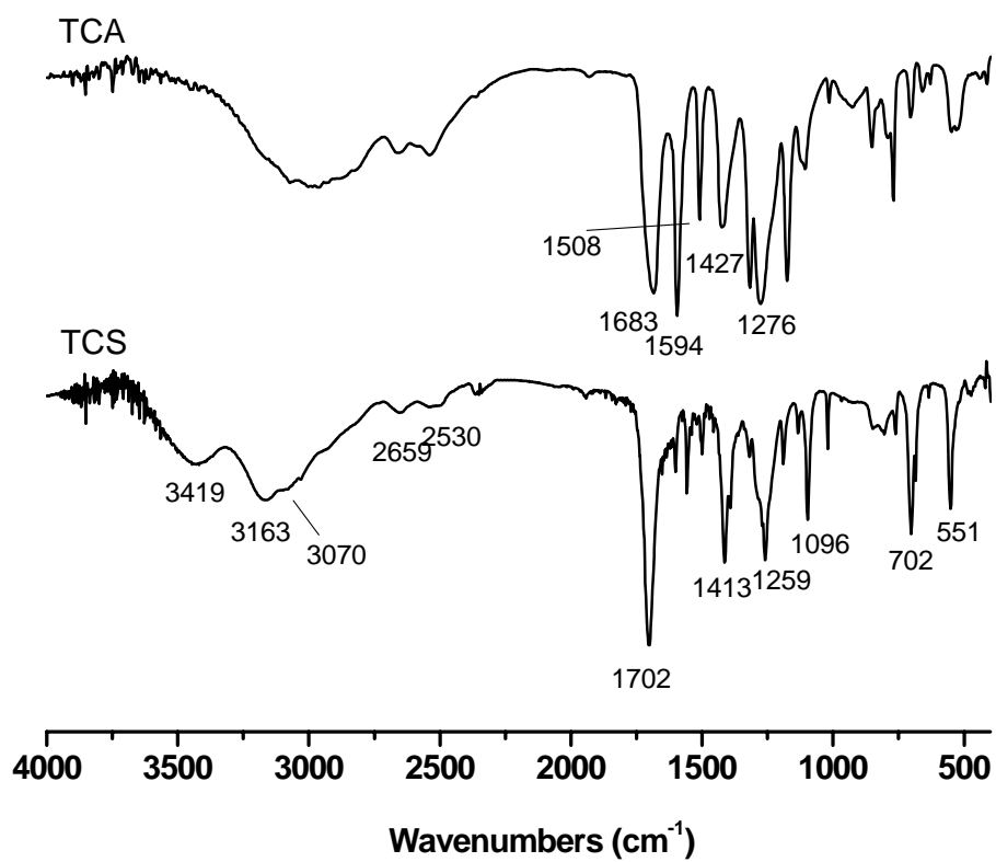
Fig. 1S FTIR spectra of TCA and TCS.
