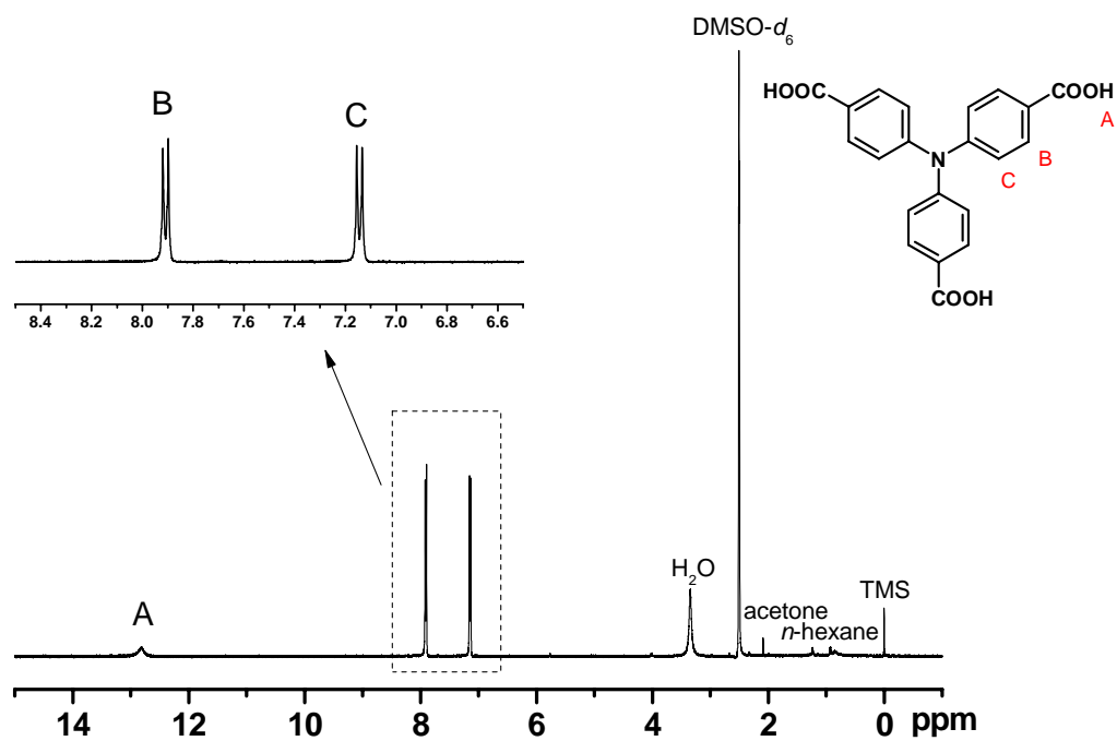
Fig. 2S ^1\text{H} NMR spectrum of TCA.
