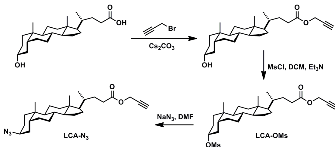
Scheme S1 The synthesis procedure of terminal alkyne and azide functionalized lithocholic acid derivatives.
