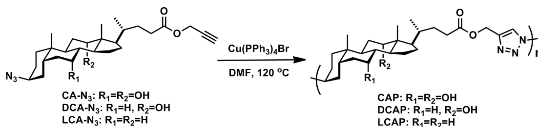
Scheme S2 The synthesis procedure of poly(bile acid)s.
