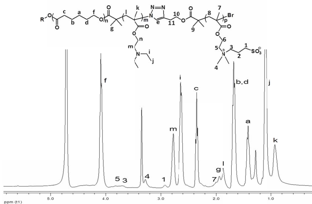
Supplementary Figure. S2 1 H NMR spectra of PCL-PDEA-PSBMA in CDCl 3 /CD 3 OD (v/v=1:1) mixture.
