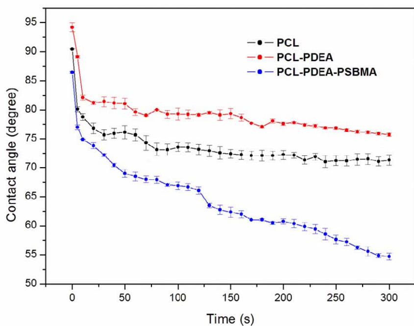
Supplementary Figure. S3 Evolution of the contact angle for PCL, PCL-PDEA and PCL-PDEA-PSBMA.
