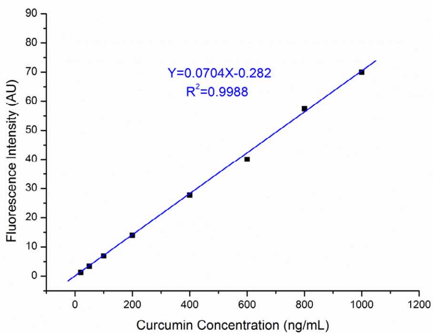
Supplementary Figure. S4 Curcumin standard curve in blood.
