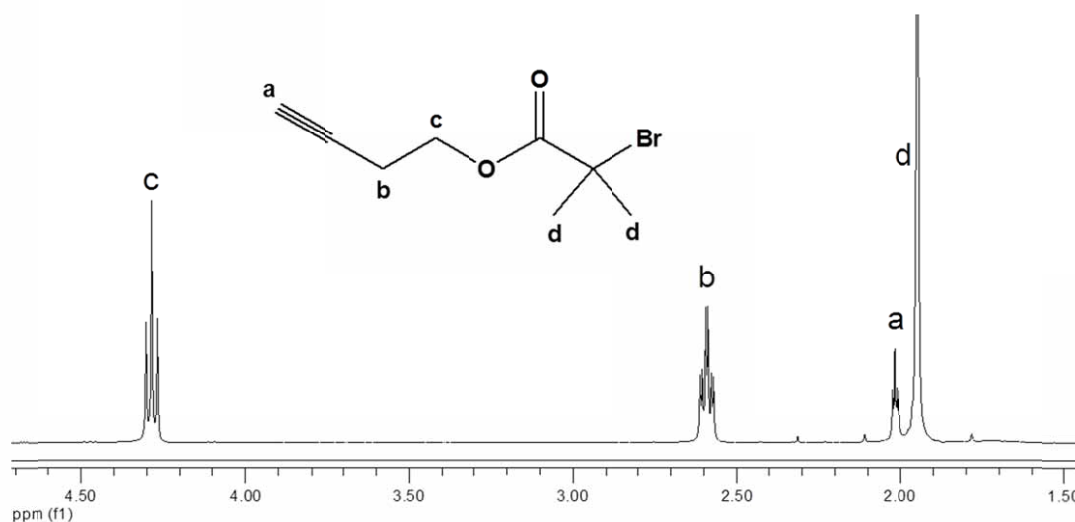
Supplementary Figure.S1 1 H NMR spectra of 3-butynyl 2-bromoisbutyrate in CDCl 3 .
