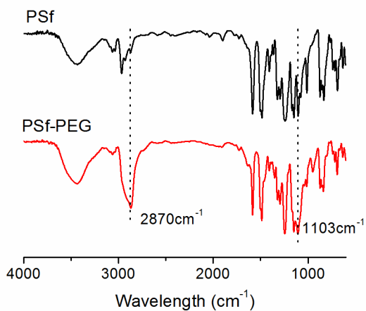
Figure S2. FTIR spectra of PSf and PSf-PEG 5000 (31.1 wt% PEG, 15.0 h).
