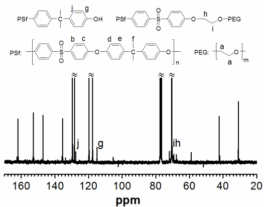
Figure S1. 13 C spectrum of PSf-PEG 5000 (31.1 wt% PEG, 15.0 h).
