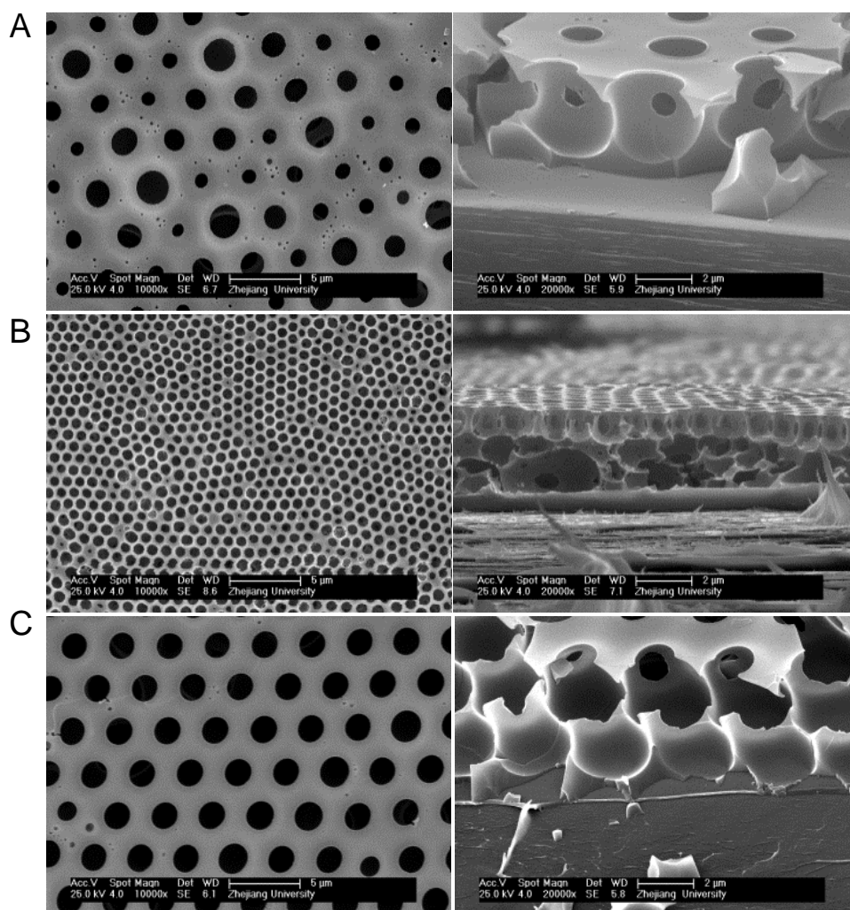
Fig. S1 Top-down (left panel) and cross-section (right panel) SEM images of honeycomb films prepared from 10 mg/mL solutions of (A) PS-cyl, (B) PS-ion, and (C) PS-neu.
