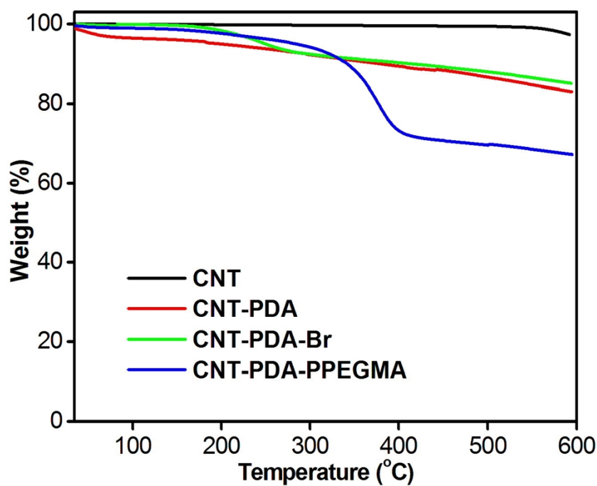
Fig. S1 TGA curves of CNTs, CNT-PDA, CNT-PDA-Br and CNT-PDA-PPEGMA
