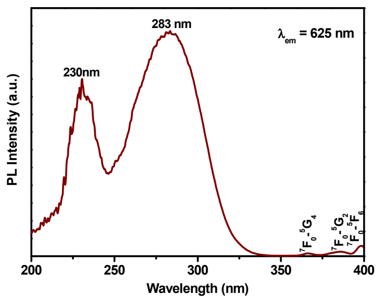
Fig. S2 Photoluminescence excitation spectra of La 2 O 3 :Eu 3+ nanowires.
