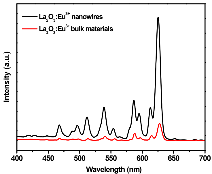
Fig. S1 A comparison of PL emission spectra of ultralong La 2 O 3 :Eu 3+ nanowires with that of La 2 O 3 :Eu 3+ bulk materials under excitation at 282 nm.
