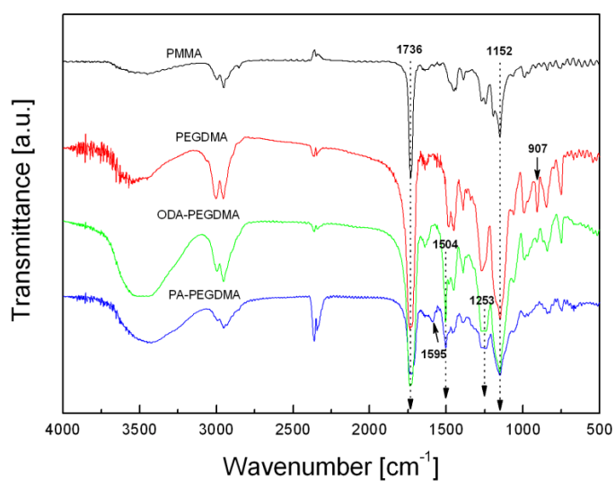
Fig. S1 FT-IR spectra of the experimental products at each step.
