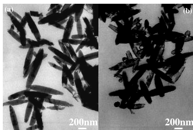
Figure S1. TEM images of the products prepared at 220 °C for (a) 12h, (b) 24h.
