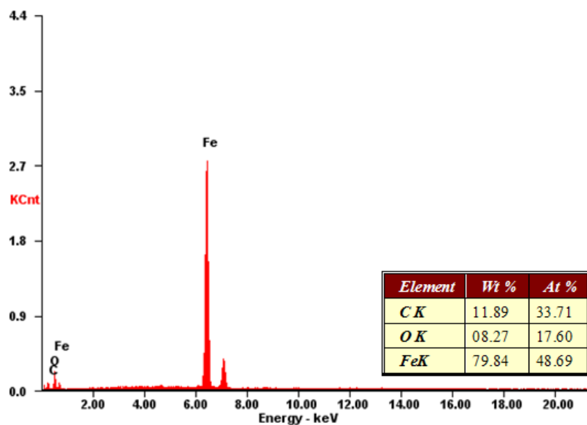
Figure S1. Energy-dispersive X-ray spectroscopy (EDX) spectrum of carbon coated Fe 3 O 4 Nanospindles
