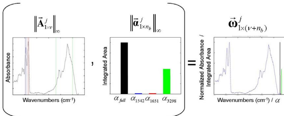
Fig. S1 Formation of concatenated vector \vec{\omega}^j from original spectrum and characteristic spectral band integrated areas
