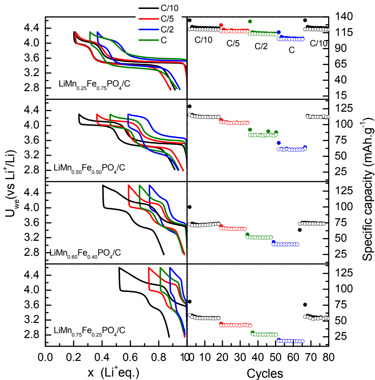
Electrochemical curves of \text{LiMn}_y\text{Fe}_{1-y}\text{PO}_4/\text{C}
