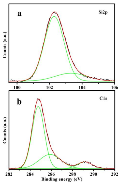
Fig. S1 XPS spectra for Si2p (a) and C1s (b) of hydrophilic SiNCs.
