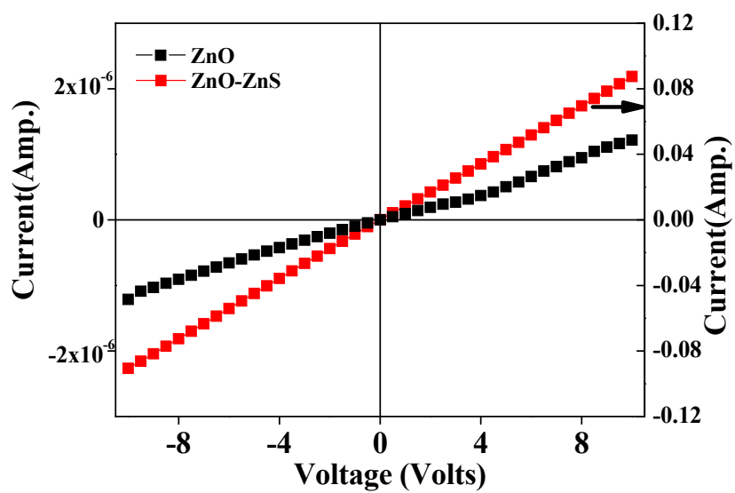
Figure S1: Current-voltage (I-V) characteristics of ITO/ZnO and ITO/ZnO/ZnS NRs arrays.
