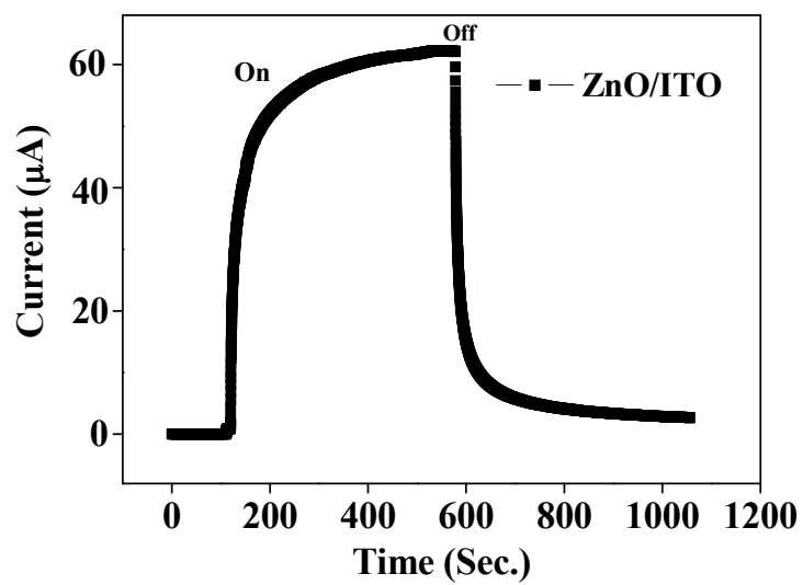
Figure S2: Photocurrent spectra of ITO/ZnO NRs arrays heterojunction.
