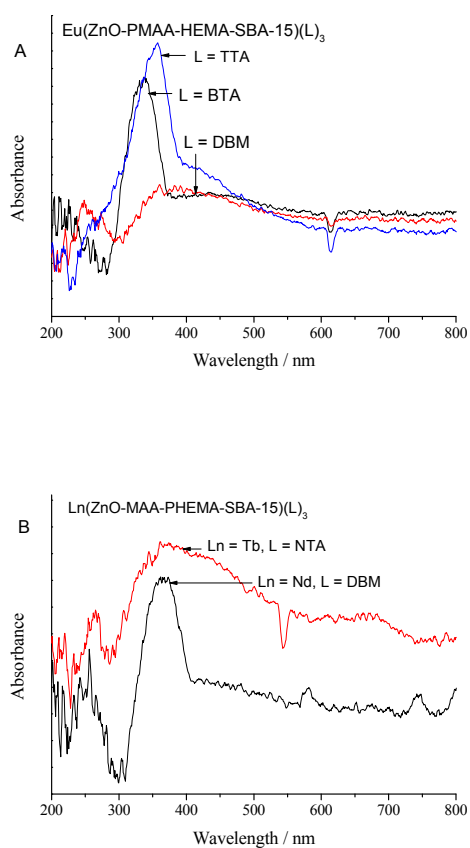
Figure S2 The ultraviolet-visible diffuse reflectance spectra of hybrid mesoporous materials: (A) europium systems, (B) terbium and neodymium system
