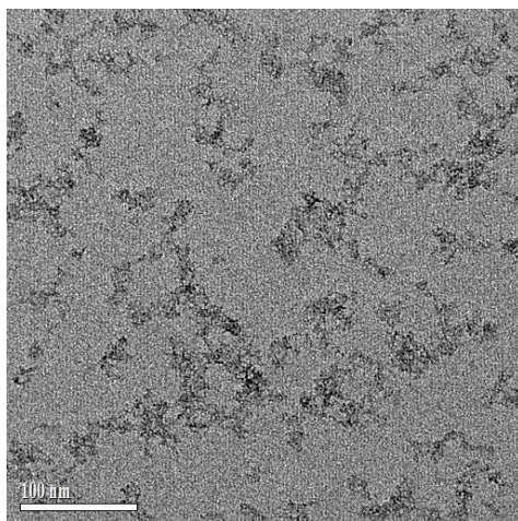
Figure S1 The selected TEM image of ZnO-MAA nanoparticles
