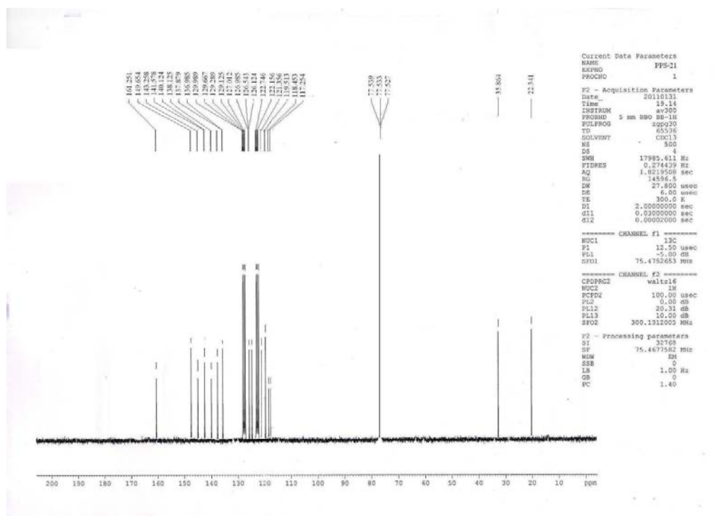
^{13}\text{C} -NMR spectrum of N,1-diphenyl-4,5-dihydro-1H-[1]benzothiepine[5,4-c]pyrazole-3-carboxamide 6,6-dioxide (12a)
