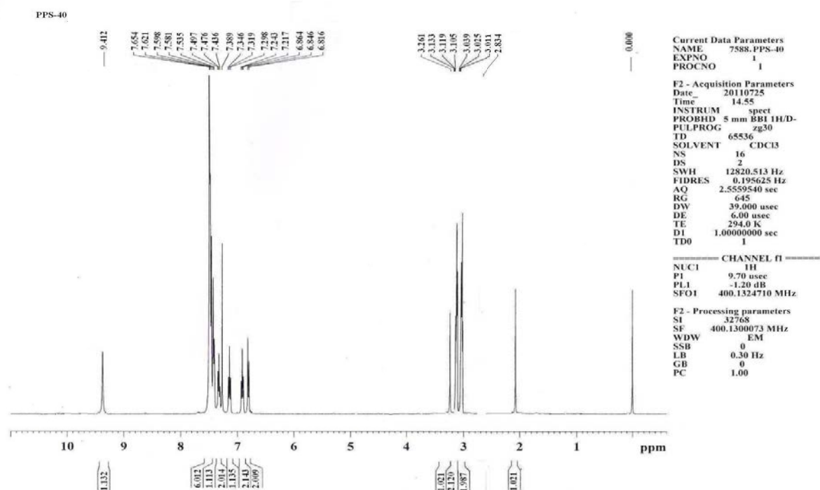
^1\text{H} -NMR spectrum of N -(1, 5-Dimethyl-3-oxo-2-phenyl-2,3-dihydro-1H-pyrazol-4-yl)-1-phenyl-4,5-dihydro-1H-[1]benzothiepine[5,4-c]pyrazole-3-carboxamide (11k)
