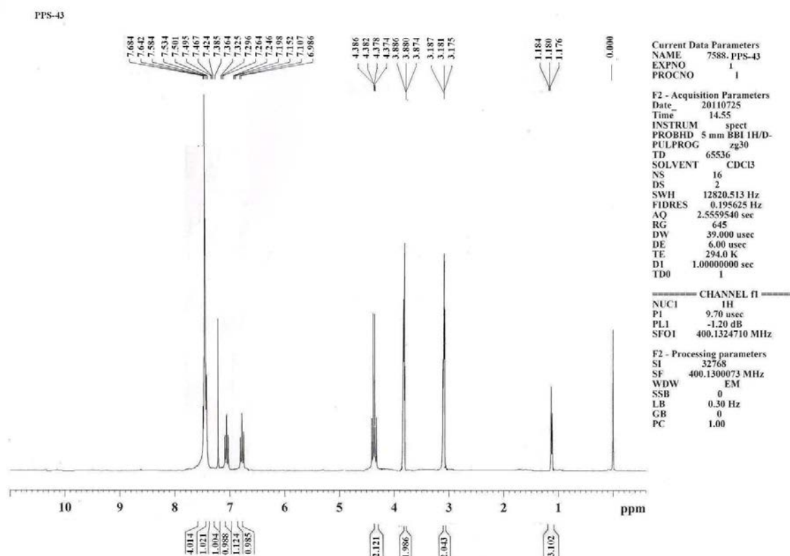
1 H-NMR spectrum of 1-(6,6-dioxido-1-phenyl-4,5-dihydro-1H-[1]benzothiepiino[5,4-c]pyrazol-3-yl)butan-1-one (8)
