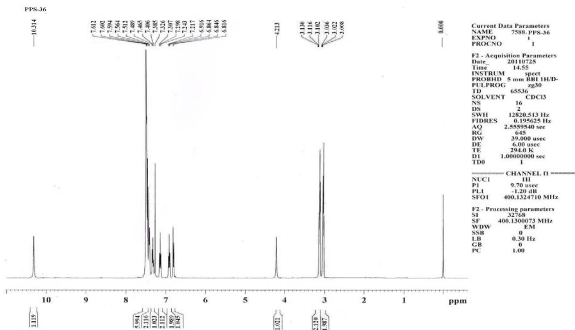
1 H-NMR spectrum of N' ,1-diphenyl-4,5-dihydro-1 H -[1]benzothiepine[5,4- c ]pyrazole-3-carbohydrazide (11j)
