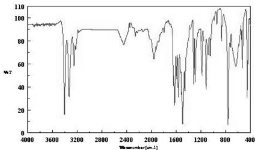
IR spectrum of N-(2-aminophenyl)-1-phenyl-4,5-dihydro-1H-[1]benzothiepine[5,4-c]pyrazole-3-carboxamide 6,6-dioxide (12h)
