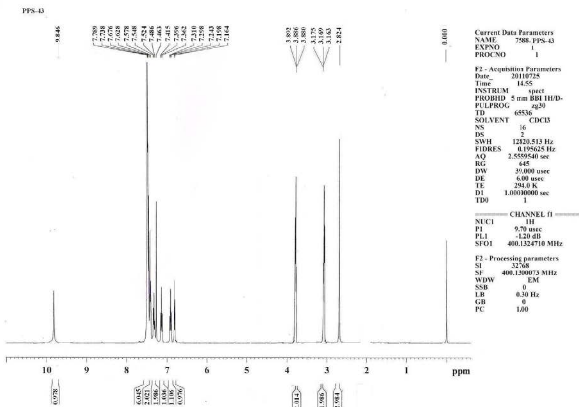
1 H-NMR spectrum of 1-Phenyl-N-p-tolyl-14,5-dihydro-1H-[1]benzothiepine[5,4-c]pyrazole-3-carboxamide 6,6-dioxide (12g)
