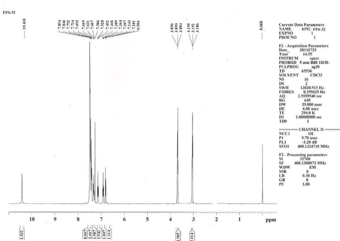
^1\text{H-NMR} spectrum of N-(Naphthalen-1-yl)-1-phenyl-4,5-dihydro-1H-[1]benzothiepine[5,4-c]pyrazole-3-carboxamide 6,6-dioxide (12m)
