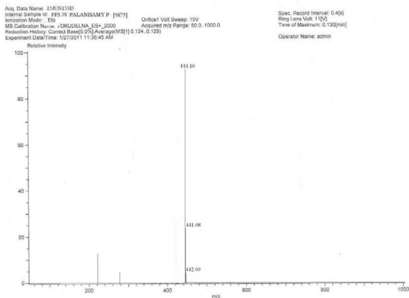
Mass spectrum of N-(2-aminophenyl)-1-phenyl-4,5-dihydro-1H-[1]benzothiepine[5,4-c]pyrazole-3-carboxamide 6,6-dioxide (12h)
