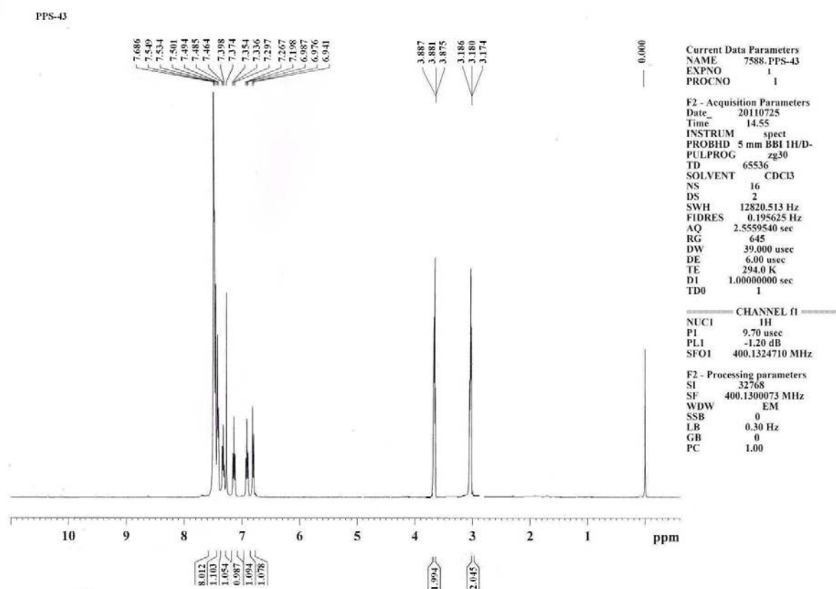
1 H-NMR spectrum of N-(1,3-benzothiazol-2-yl)-1-phenyl-4,5-dihydro-1H-[1]benzothiepine[5,4-c]pyrazole-3-carboxamide 6,6-dioxide (12)
