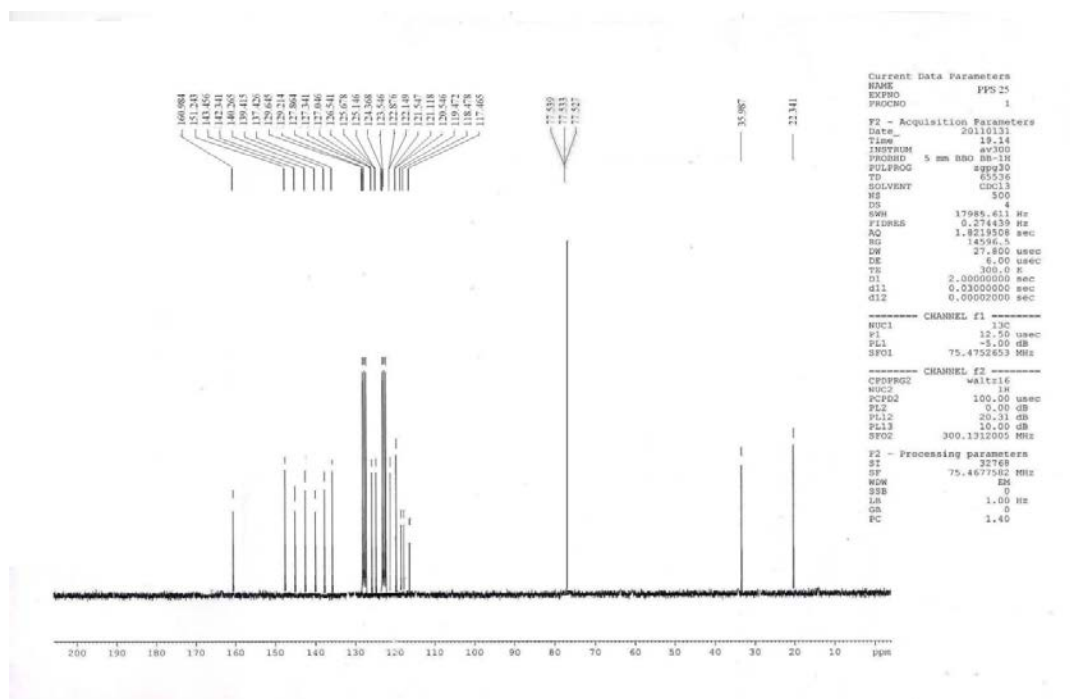
13 C-NMR spectrum of N -(Naphthalen-1-yl)-1-phenyl-4,5-dihydro-1 H -[1]benzothiepine[5,4- c ]pyrazole-3-carboxamide (11m)
