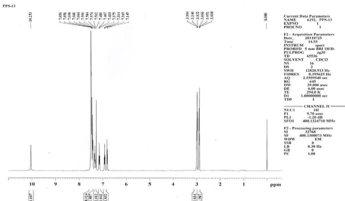
1 H-NMR spectrum of N -(4-nitrophenyl)-1-phenyl-4,5-dihydro-1 H -[1]benzothiepine[5,4- c ]pyrazole-3-carboxamide (11e)
