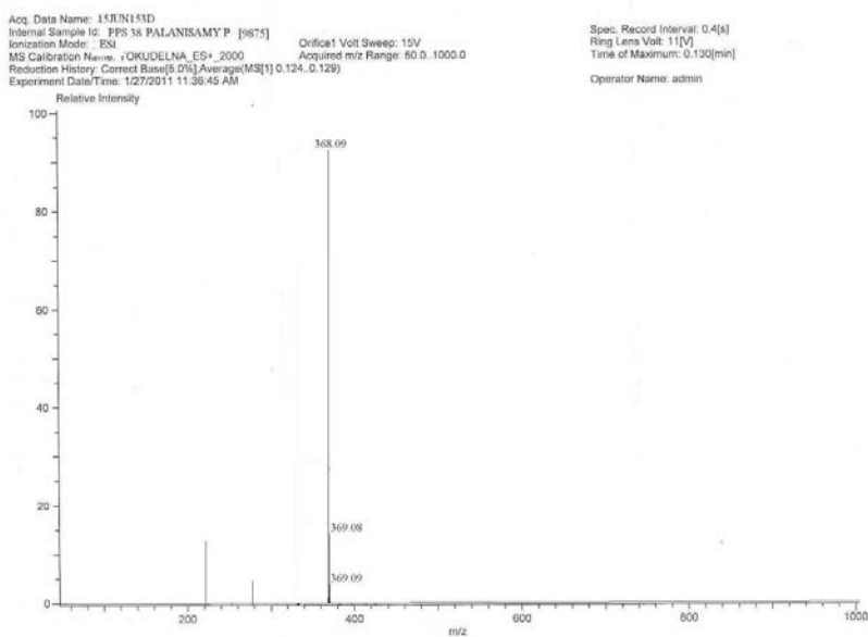
Mass spectrum of 1-phenyl-4,5-dihydro-1H-[1]benzothiepine[5,4-c]pyrazole-3-carbohydrazide 6,6-dioxide (12i)
