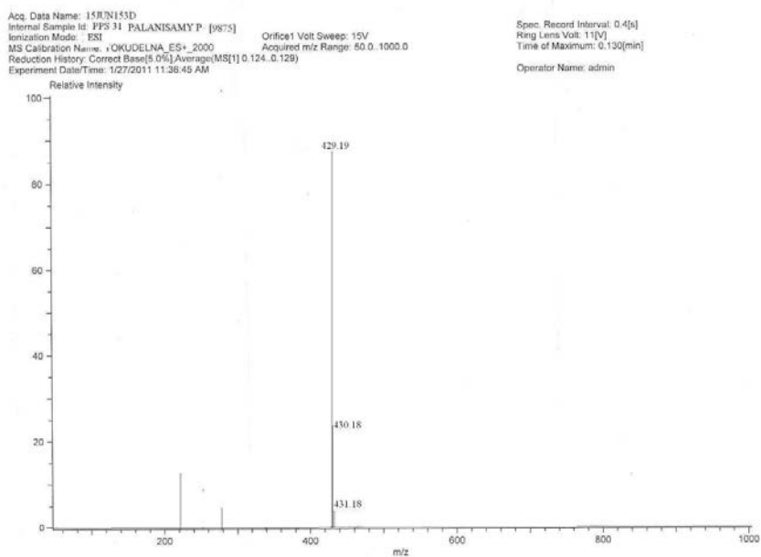
Mass spectrum of N,1-diphenyl-4,5-dihydro-1H-[1]benzothiepine[5,4-c]pyrazole-3-carboxamide 6,6-dioxide (12a)
