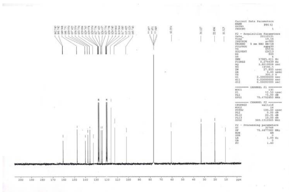
13 C-NMR spectrum of N-(1, 5-Dimethyl-3-oxo-2-phenyl-2,3-dihydro-1H-pyrazol-4-yl)-1-phenyl-4,5-dihydro-1H-[1]benzothiepiino[5,4-c]pyrazole-3-carboxamide 6,6-dioxide (12k)
