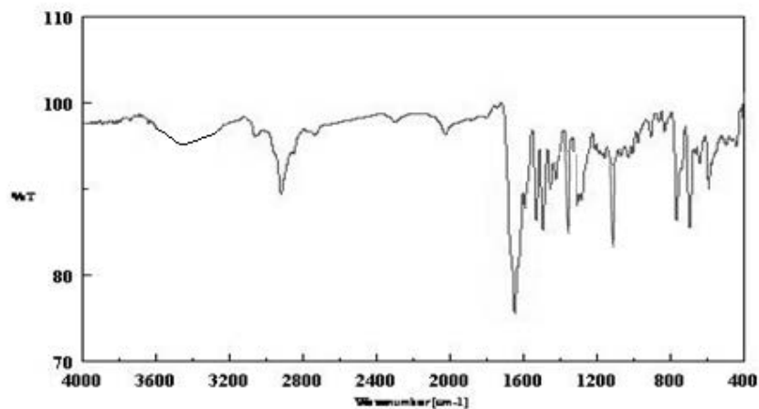
IR spectrum of N-(1, 5-Dimethyl-3-oxo-2-phenyl-2,3-dihydro-1H-pyrazol-4-yl)-1-phenyl-4,5-dihydro-1H-[1]benzothiepine[5,4-c]pyrazole-3-carboxamide 6,6-dioxide (12k)
