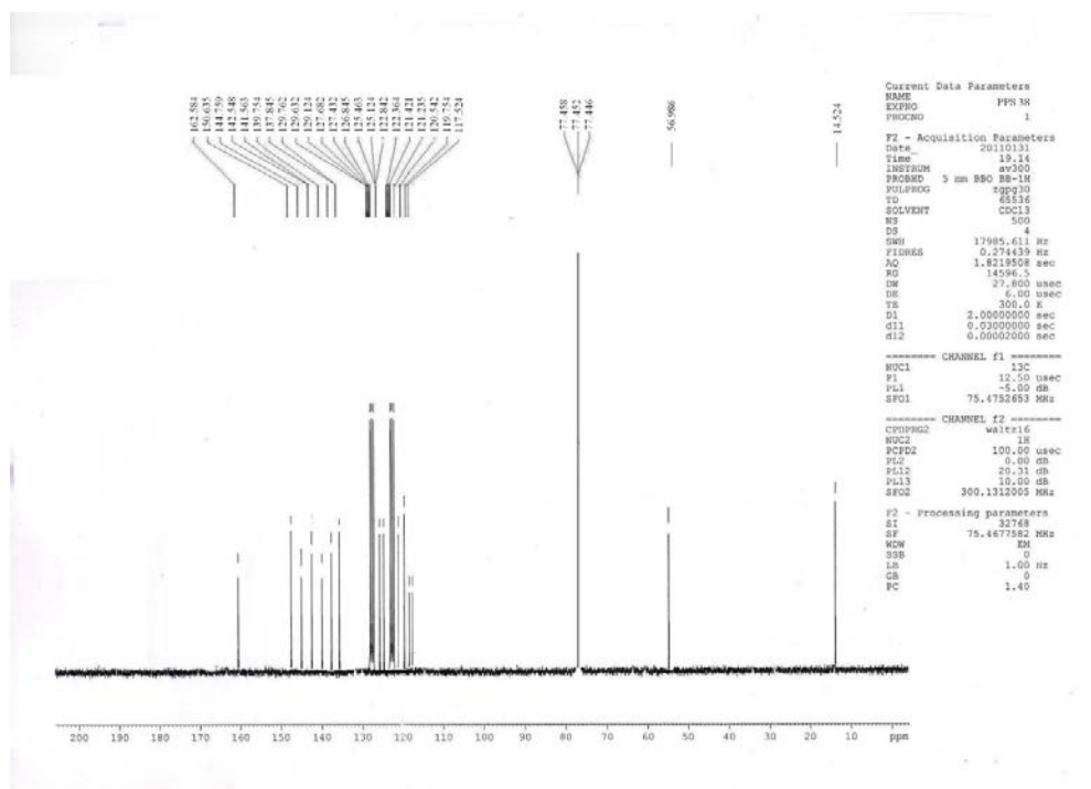
13 C-NMR spectrum of N-(4-nitrophenyl)-1-phenyl-4,5-dihydro-1H-[1] benzothiepine[5,4-c]pyrazole-3-carboxamide 6,6-dioxide (12e)
