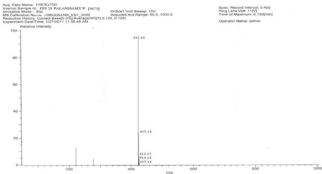
Mass spectrum of N' ,1-diphenyl-4,5-dihydro-1 H -[1]benzothiepine[5,4- c ]pyrazole-3-carbohydrazide (11j)
