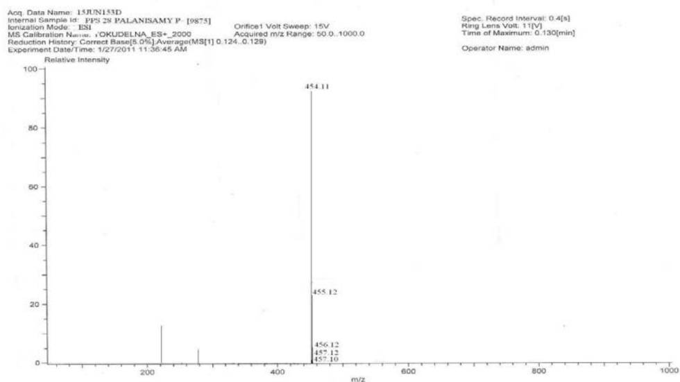
Mass spectrum of N -(1,3-benzothiazol-2-yl)-1-phenyl-4,5-dihydro-1 H -[1]benzothiepine[5,4- c ]pyrazole-3-carboxamide (11)
