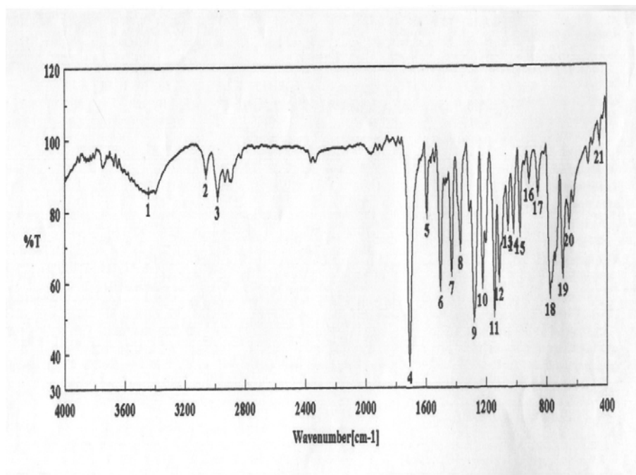
IR spectrum of ethyl 1-phenyl-4,5-dihydro-1 H -[1]benzothiepine[5,4- c ]pyrazole-3-carboxylate (7)
