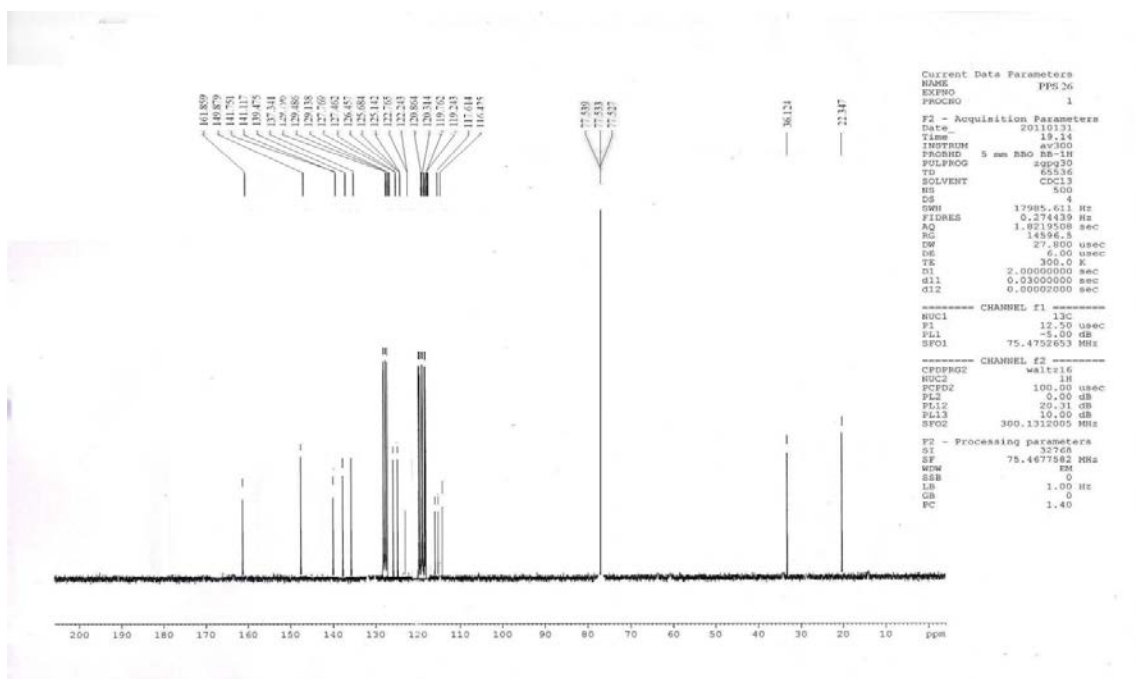
13 C-NMR spectrum of N -(2-aminophenyl)-1-phenyl-4,5-dihydro-1 H - [1]benzothiepine[5,4- c ]pyrazole-3-carboxamide (11h)
