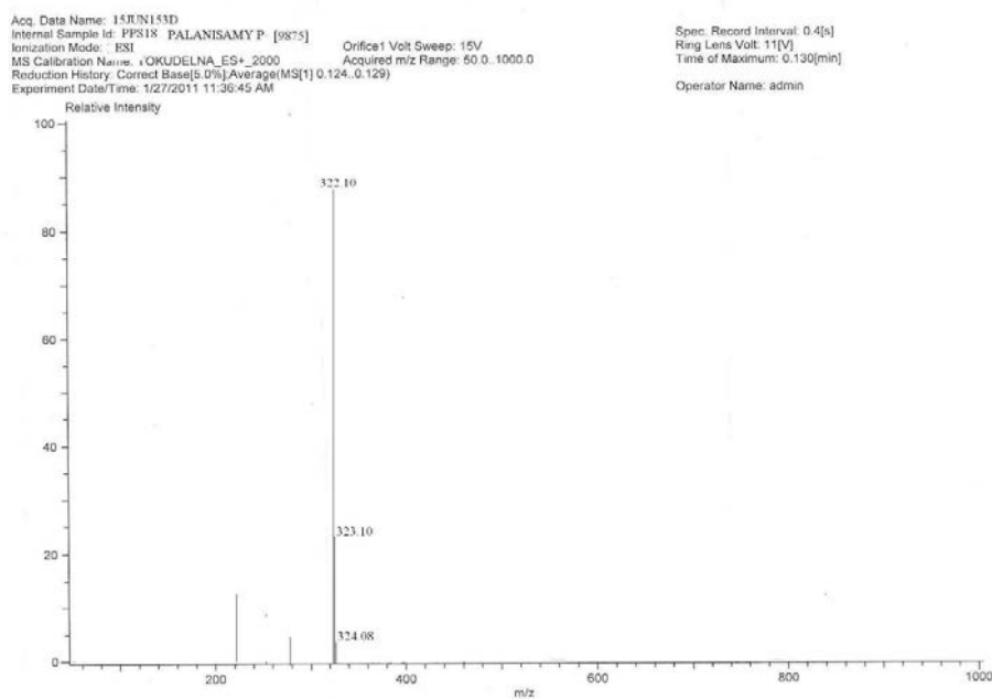
Mass spectrum of 1-phenyl-4,5-dihydro-1 H -[1]benzothiepine[5,4- c ]pyrazole-3-carboxylic acid (9)
