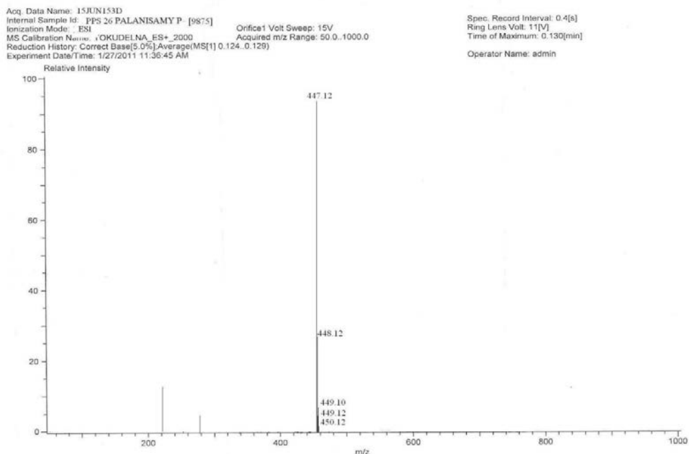
Mass spectrum of N -(Naphthalen-1-yl)-1-phenyl-4,5-dihydro-1 H -[1]benzothiepine[5,4- c ]pyrazole-3-carboxamide (11m)
