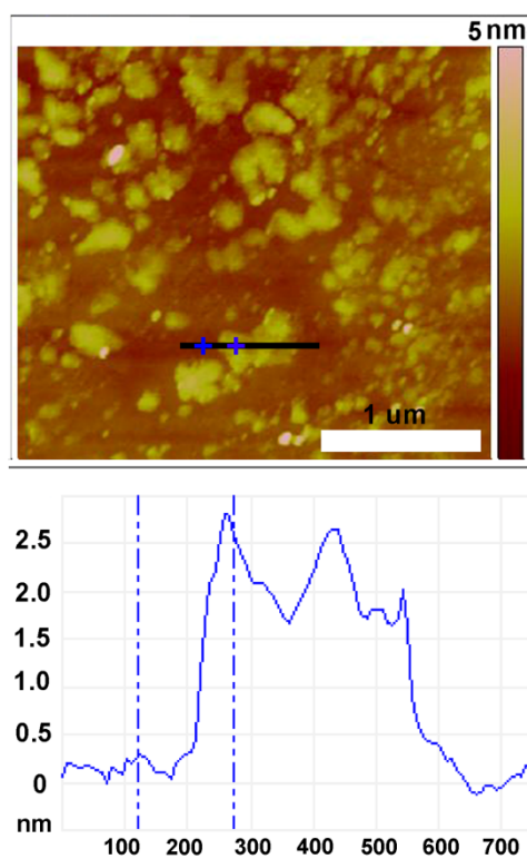
Fig. S1 AFM image and height distribution histograms of [BMI]-GONs on a silicon substrate.
