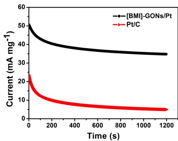
Fig. S3 Chronoamperometry curves for [BMI]-GONs/Pt and Pt/C in 0.5 M H 2 SO 4 .
