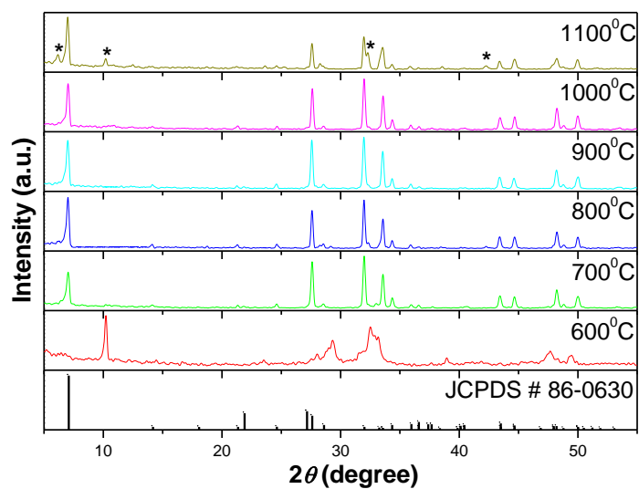
Fig. S1 XRD patterns of samples \text{NaGd}_{0.7}\text{Eu}_{0.3}\text{TiO}_4 annealed at different temperature for 6 h in air (* indicates the \text{Na}_2\text{Gd}_2\text{Ti}_3\text{O}_{10} peak).
