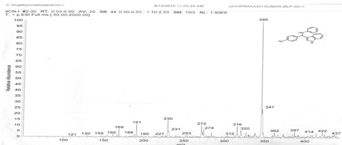
Fig. 24 ESI Mass Spectra of compound 4Ah
