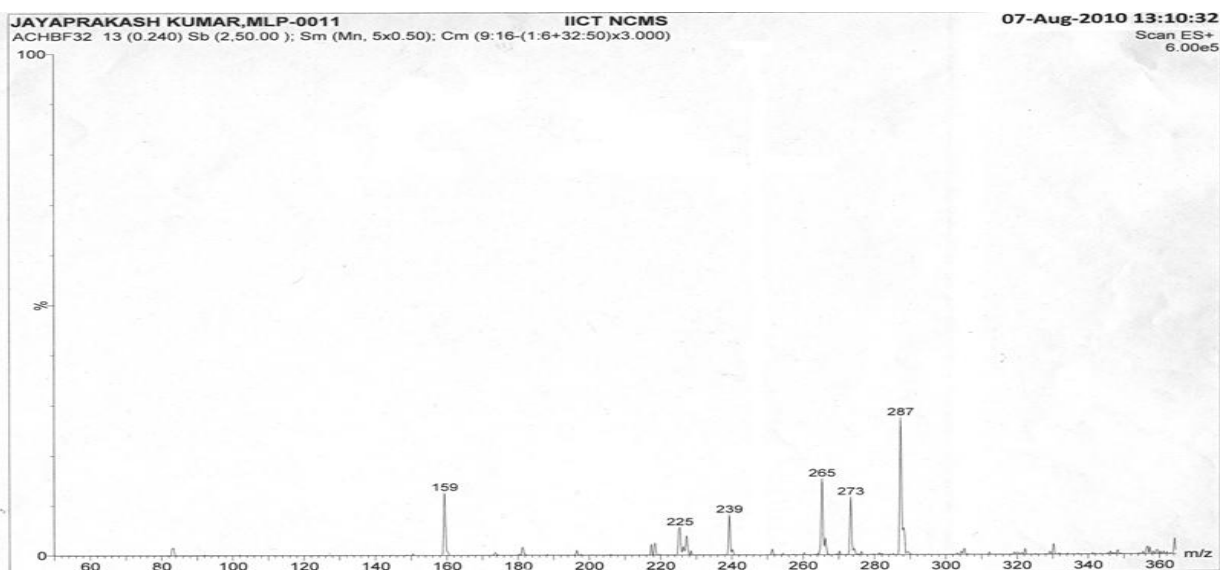
Fig. 39 ESI Mass Spectra of compound 4E
