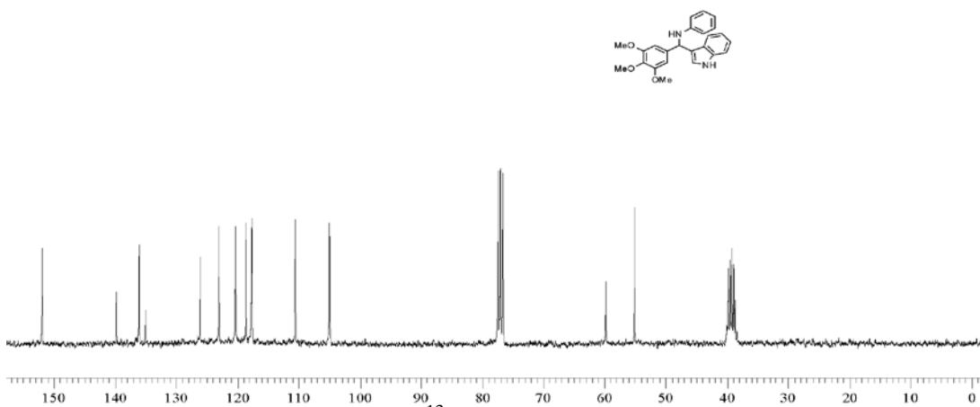
Fig. 14 13 C NMR of compound 4Ae
