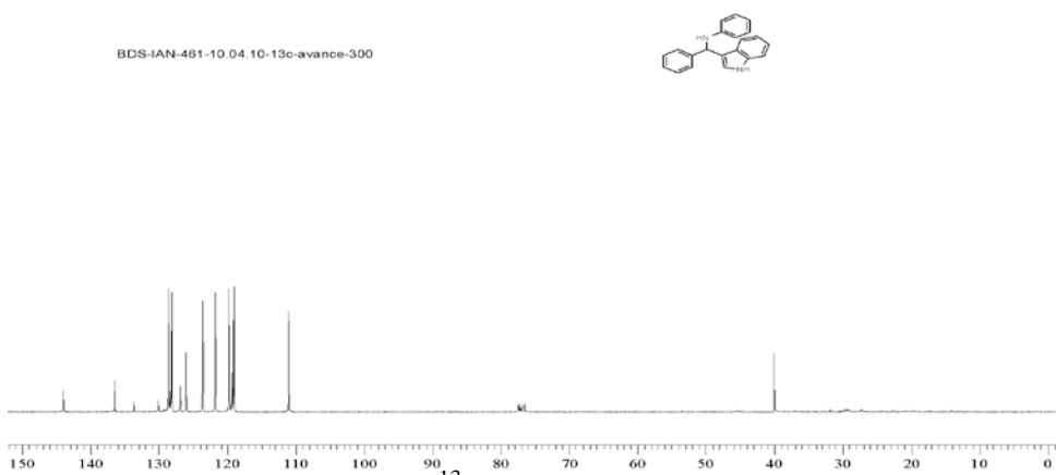
Fig. 2 ^{13}\text{C} NMR of compound 4Aa
