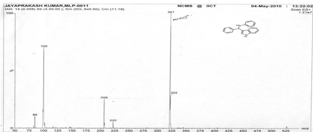
Fig. 3 ESI Mass Spectra of compound 4Aa
