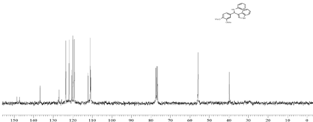
Fig. 11 13 C NMR of compound 4Ad
