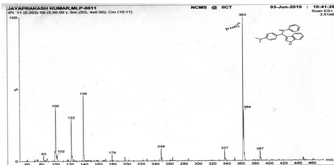
Fig. 9 ESI Mass Spectra of compound 4Ac
