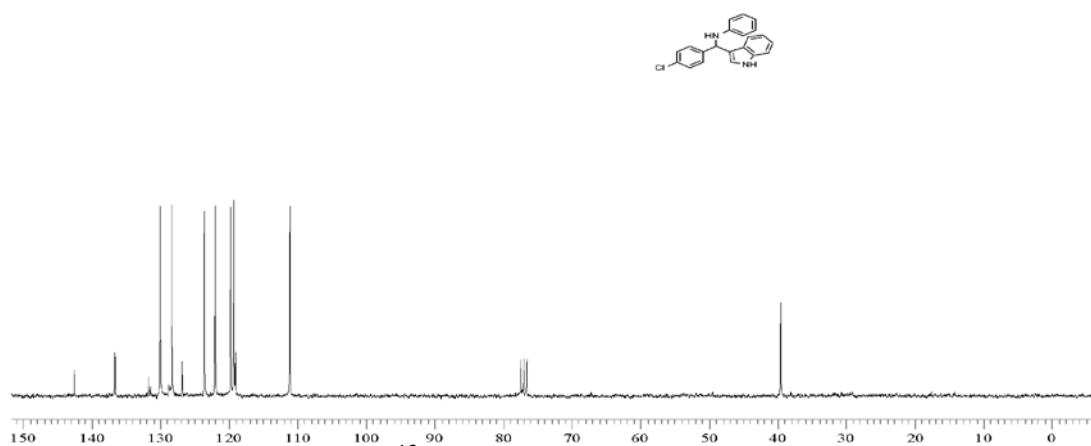
Fig. 17 13 C NMR of compound 4Af
