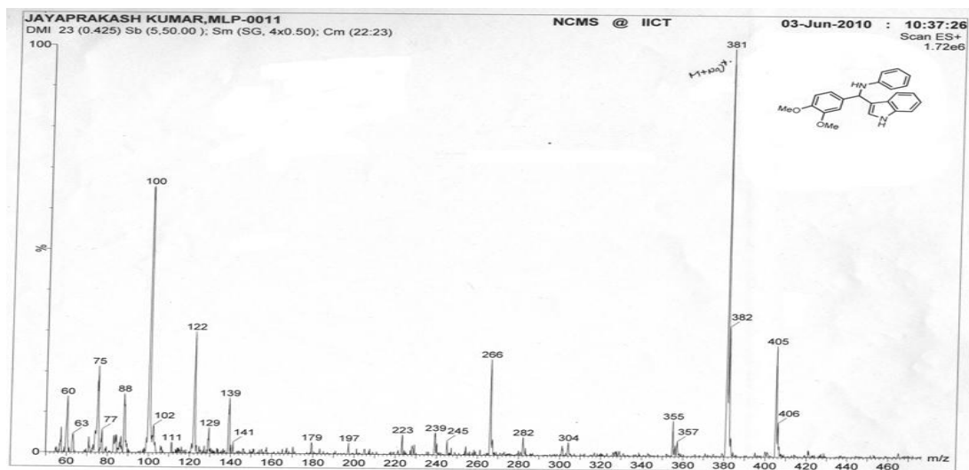
Fig. 12 ESI Mass Spectra of compound 4Ad
