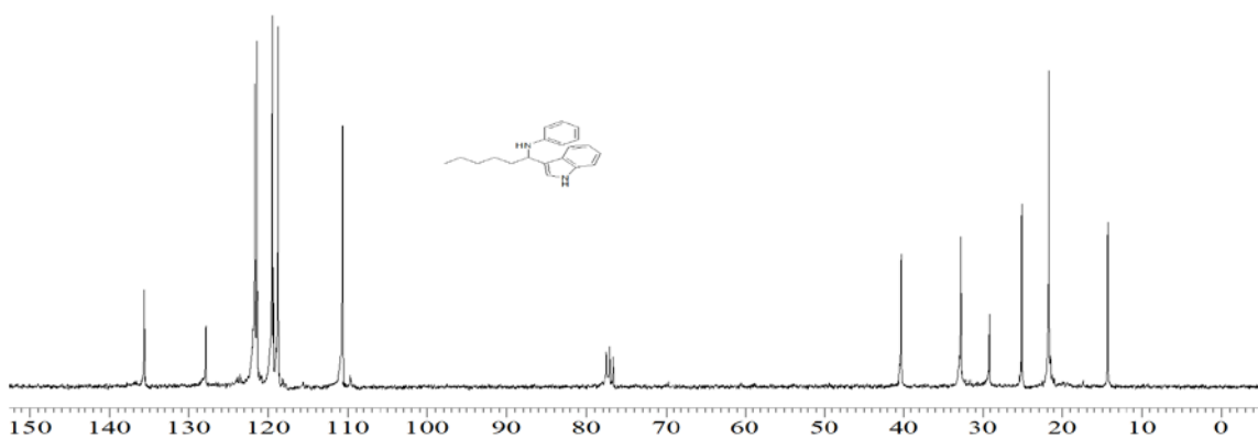
Fig. 35 13 C NMR of compound 4D
