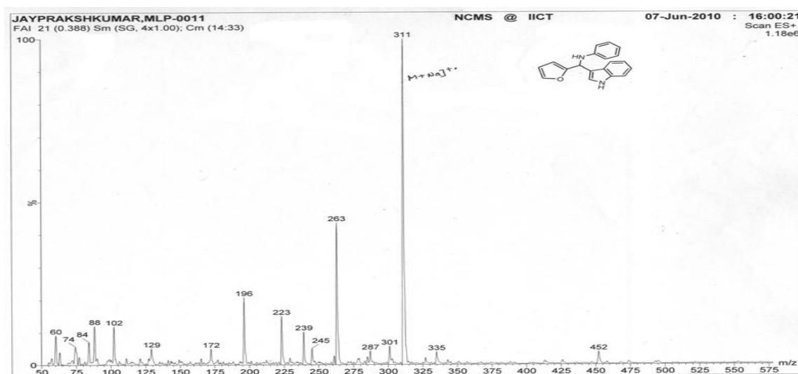
Fig. 30 ESI Mass Spectra of compound 4B
