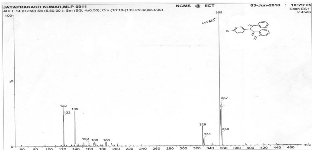
Fig. 18 ESI Mass Spectra of compound 4Af
