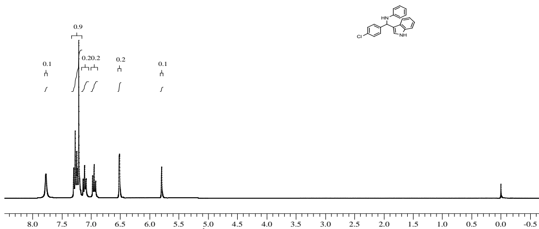
Fig. 16 1 H NMR of compound 4Af
