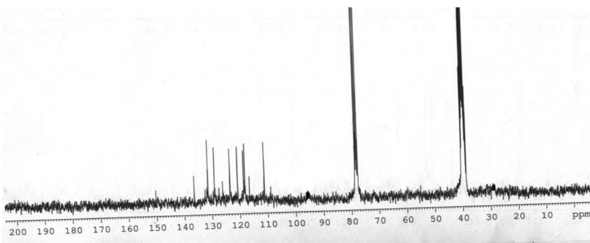
Fig. 23 13 C NMR of compound 4Ah
