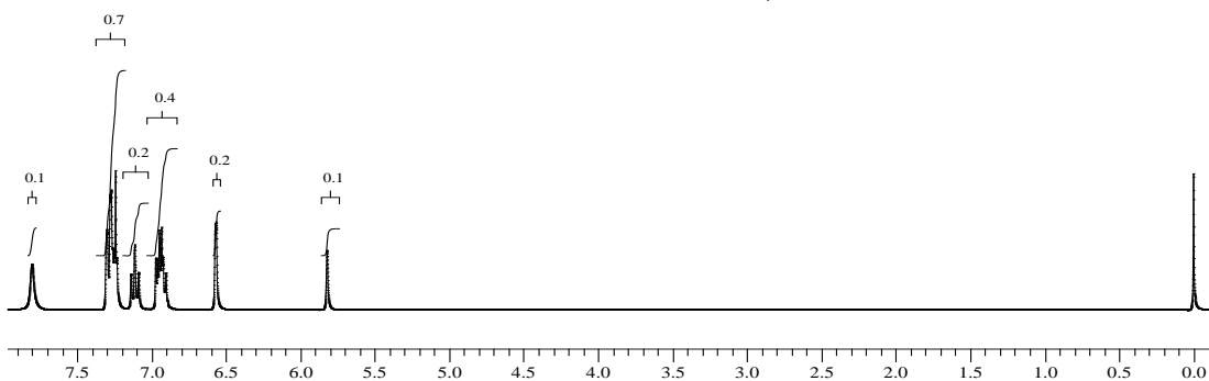
Fig. 19 ^1\text{H} NMR of compound 4Ag
