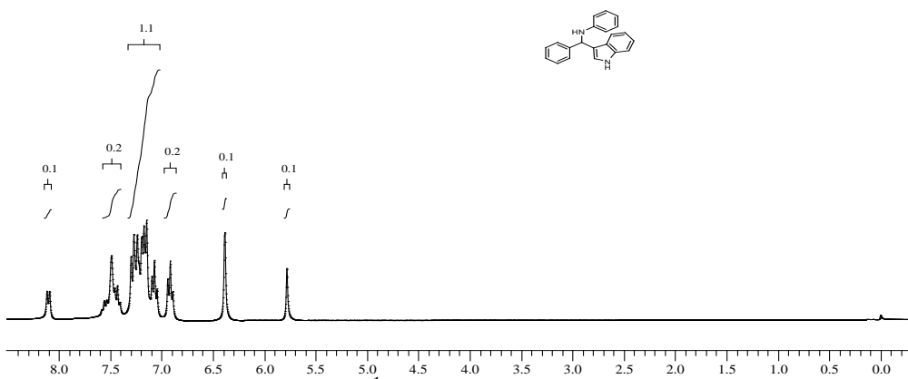
Fig. 1 ^1\text{H} NMR of compound 4Aa
