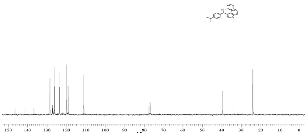
Fig. 8 13 C NMR of compound 4Ac
