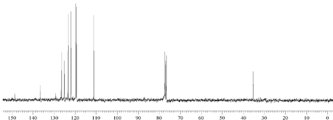
Fig. 32 ^{13}\text{C} NMR of compound 4C
