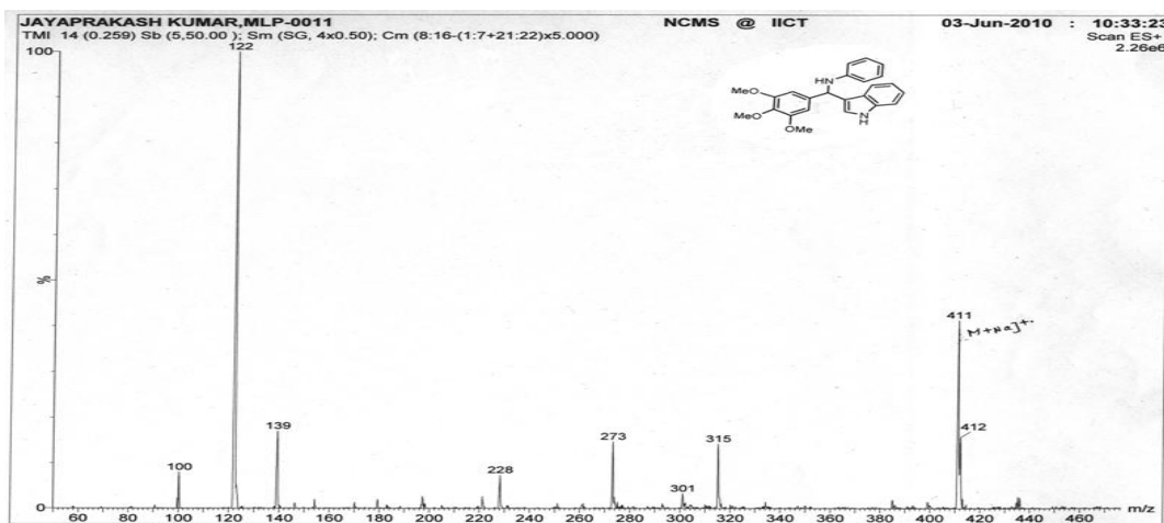
Fig. 15 ESI Mass Spectra of compound 4Ae
