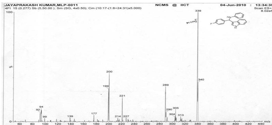
Fig. 21 ESI Mass Spectra of compound 4Ag
