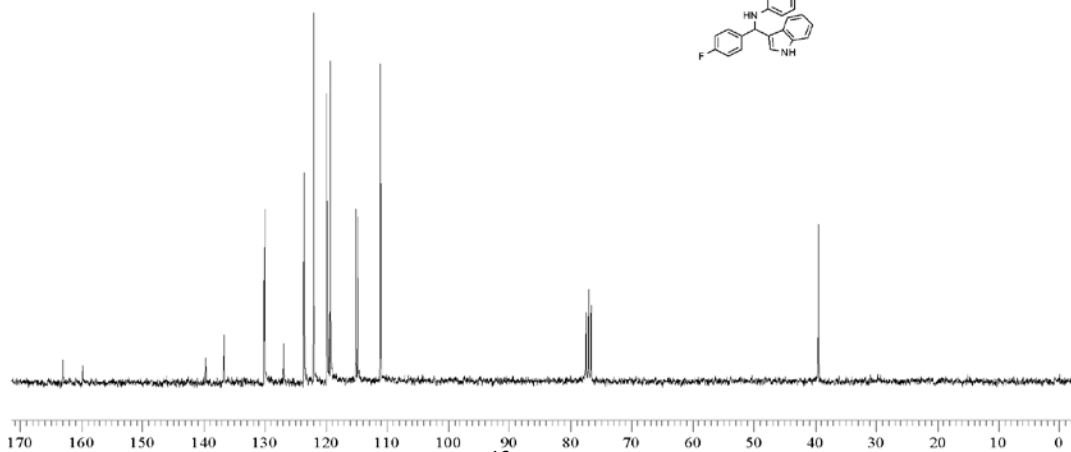
Fig. 20 ^{13}\text{C} NMR of compound 4Ag
