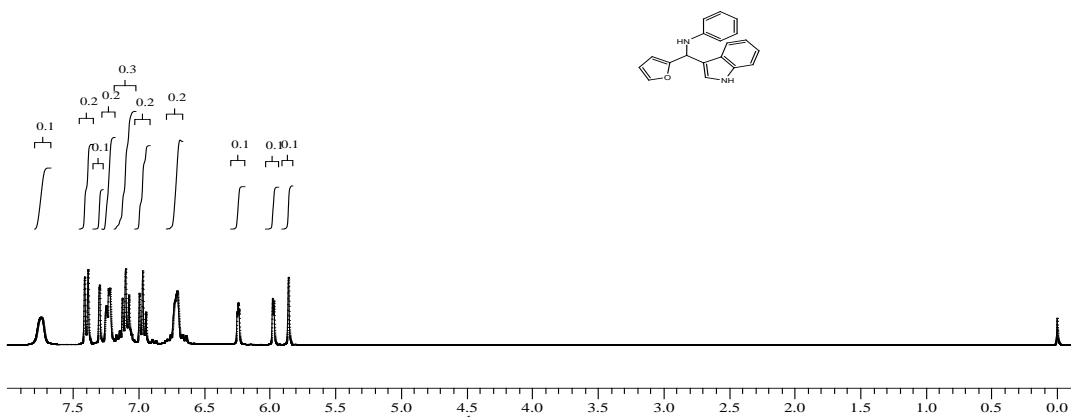
Fig. 28 1 H NMR of compound 4B
