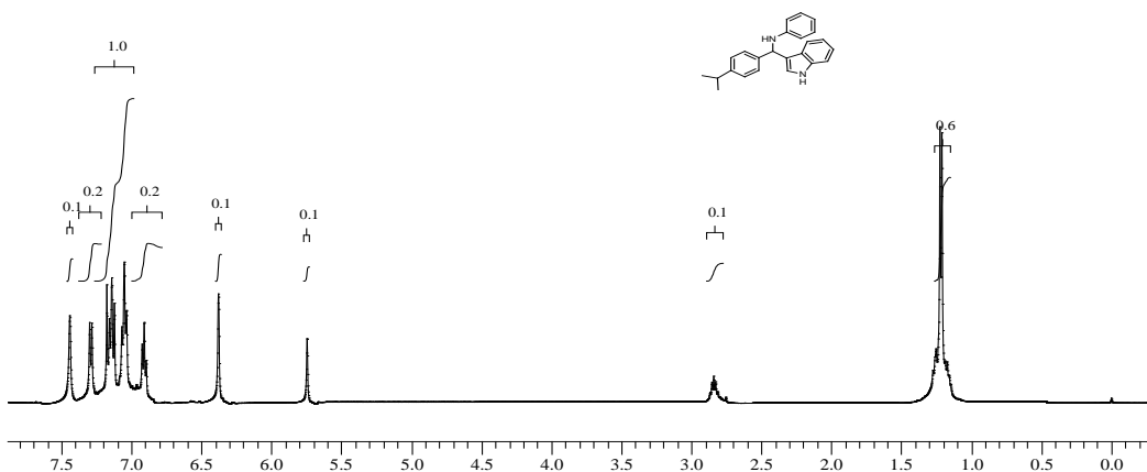
Fig. 7 1 H NMR of compound 4Ac
