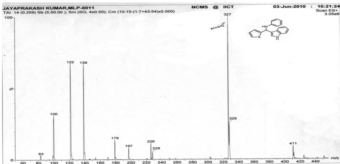
Fig. 33 ESI Mass Spectra of compound 4C
