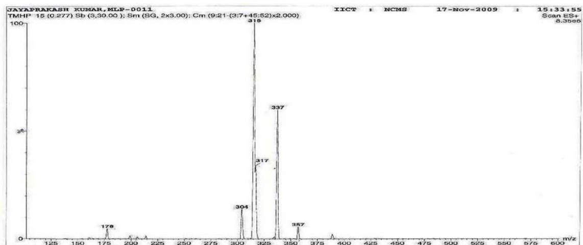
Fig. 36 ESI Mass Spectra of compound 4D
