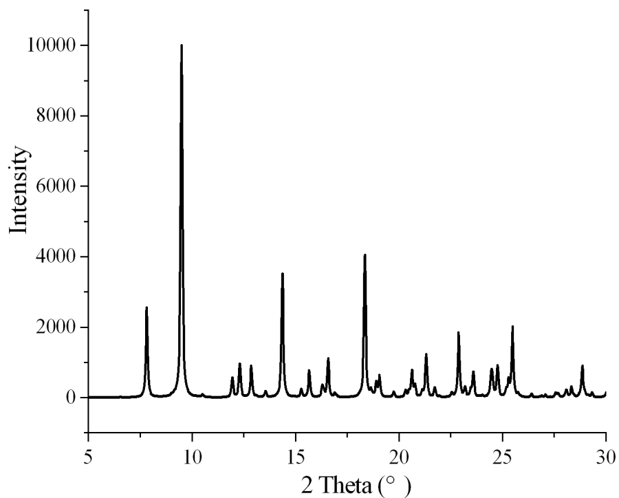
Fig. S1 The simulated PXRD pattern of the [\text{Mn}(\text{CuL})_3(\text{ClO}_4)_2]_n crystal reported in ref. 43.
