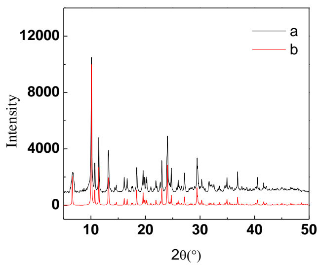
Fig. S10 XRD spectrograms of complexes 5
