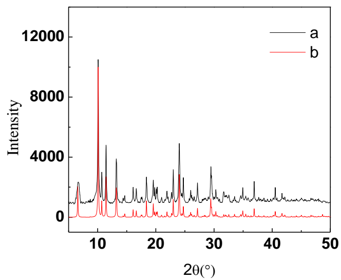
Fig. S9 XRD spectrograms of complexes 4
