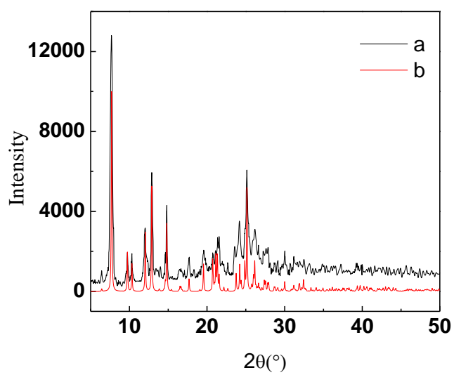
Fig. S8 XRD spectrograms of complexes 3
