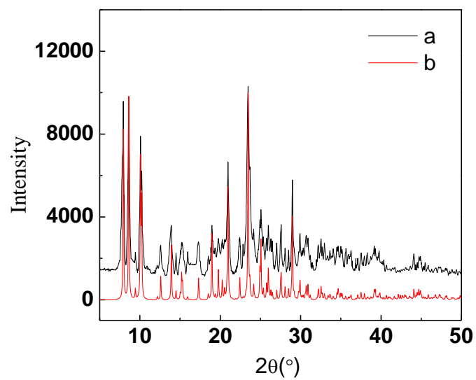
Fig. S6 XRD spectrograms of complexes 1
