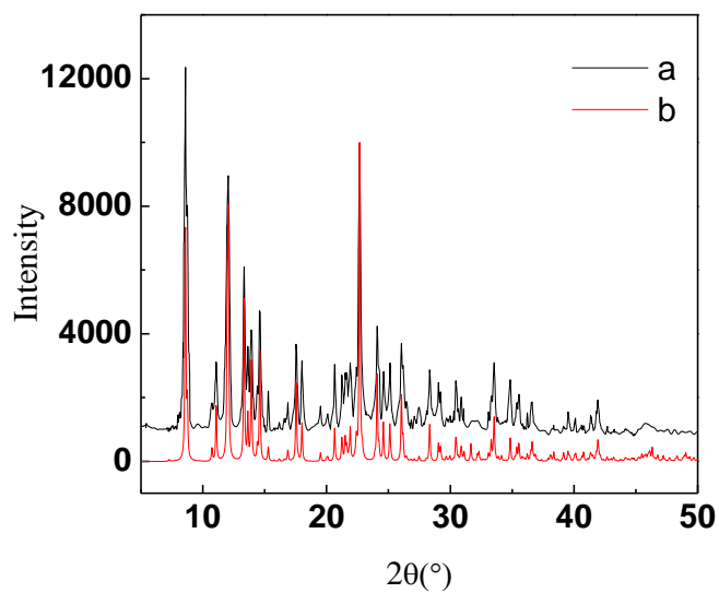
Fig. S7 XRD spectrograms of complexes 2
