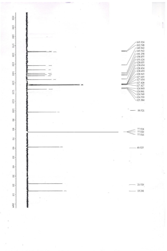
Fig. 4.27 ^1\text{H-NMR} ( \text{DMSO-}d_6 ) spectrum of ethyl 2,3-diphenyl-2,3-dihydro-1H-thiochromeno[5,4-thiochromeno]5,4-c[diazepine-5-carboxylate (9)
