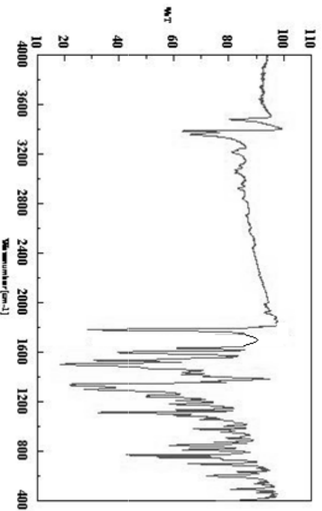
Fig. 4.45 IR (KBr) spectrum of ethyl 2-thioxo-1,2,5,6-tetrahydro[1]benzothiepinol[5,4-d]pyrimidine-4-carboxylate (16)
