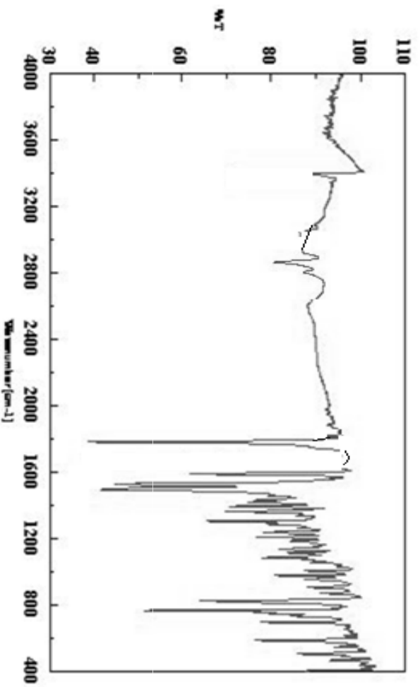
Fig. 4.25 IR (KBr) spectrum of ethyl 2,3-diphenyl-2,3-dihydro-1H-thiochromeno[5,4-c]diazepine-5-carboxylate (9)
