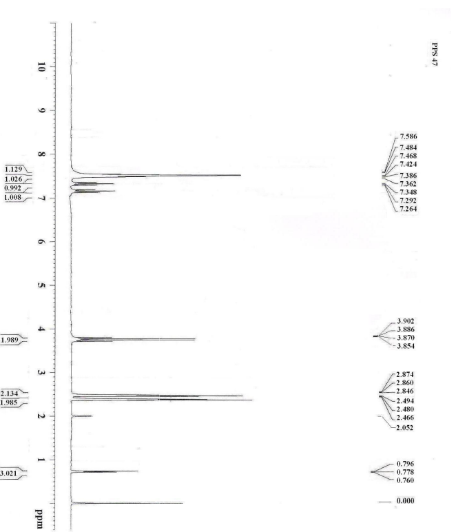
Fig. 4.46 1 H-NMR (CDCl 3 , DMSO-d 6 ) spectrum of Ethyl 2-thioxo-1,2,5,6-tetrahydro[1]benzothiepinol[5,4-d]pyrimidine-4-carboxylate (16)
