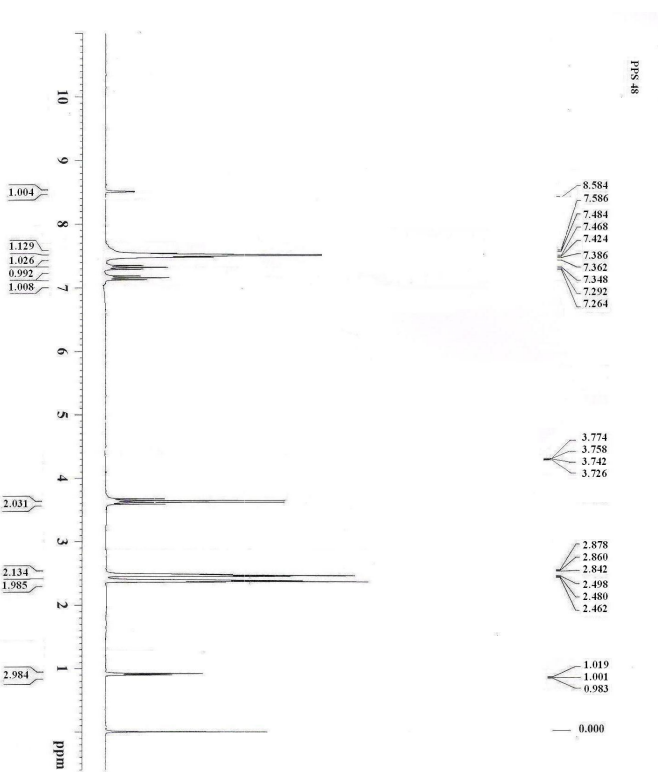
Fig. 4.42 1 H-NMR (DMSO-d 6 ) spectrum of ethyl 2-oxo-1,2,5,6-tetrahydro[1]benzothiepinol[5,4-d]pyrimidine-4-carboxylate (15)
