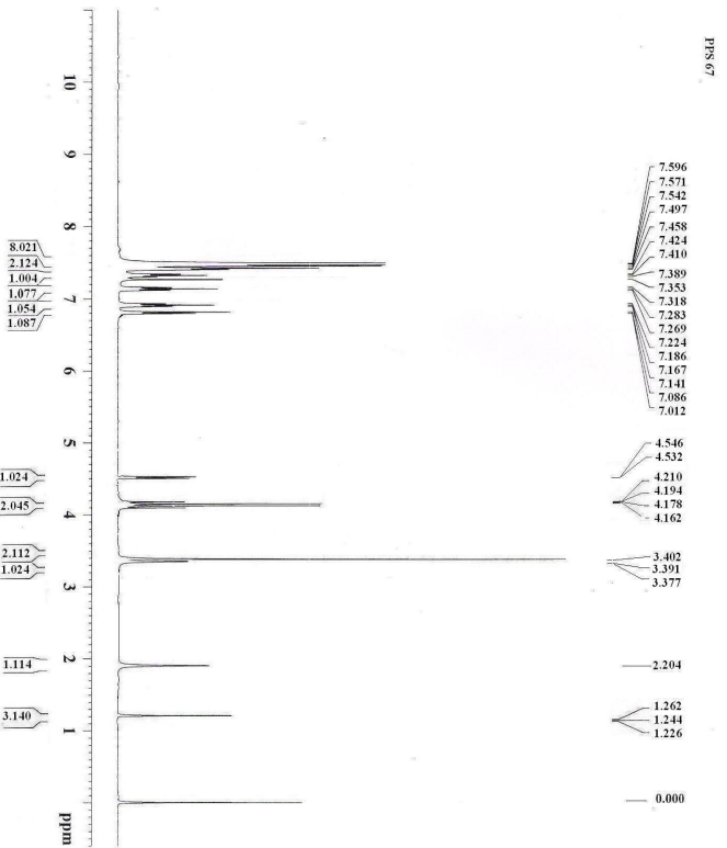
Fig. 4.26 1 H-NMR (CDCl 3 ) spectrum of ethyl 2,3-diphenyl-2,3-dihydro-1H-thiochromeno[5,4-c]diazepine-5-carboxylate (9)
