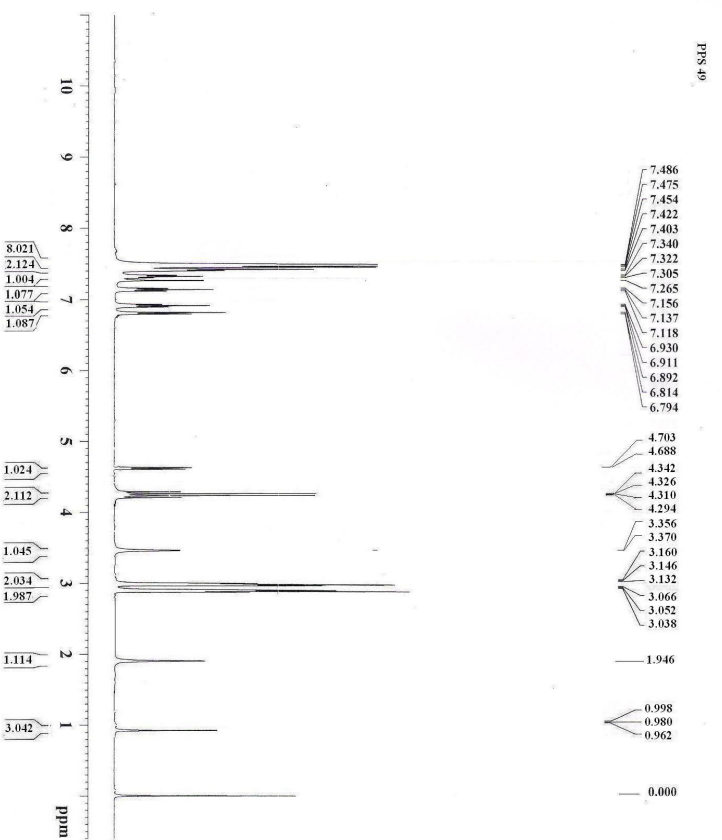
Fig. 4.54 1H-NMR (DMSO-d6) spectrum of ethyl 2,3-diphenyl-2,3-dihydro-1H-benzothiepine [5,4-c]diazepine-5-carboxylate (18)
