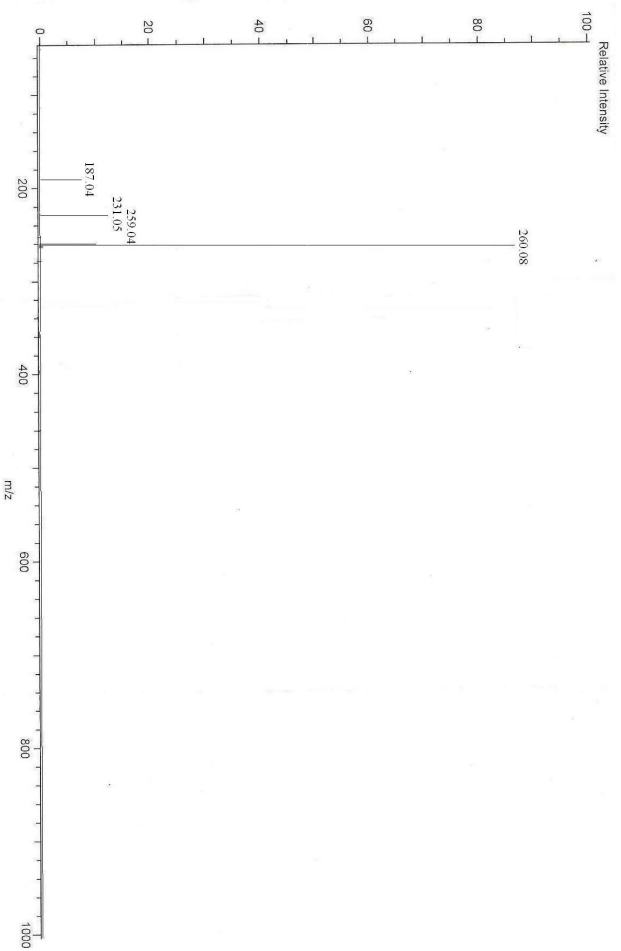
Fig. 4.8 Mass (ESI) spectrum of ethyl 1,4-dihydrothiochromeno[4,3-c]pyrazole-3-carboxylate (4)
