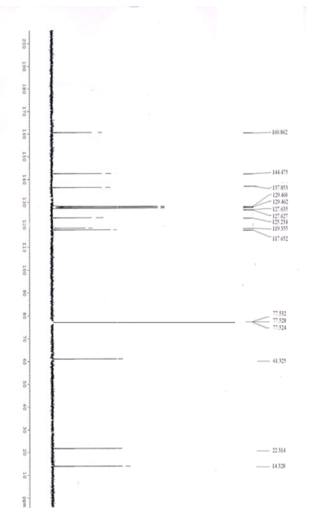
Fig. 4.7 13 C-NMR (CDCl 3 ) spectrum of ethyl 1,4-dihydrothiochromeno[4,3-c]pyrazole-3-carboxylate (4)
