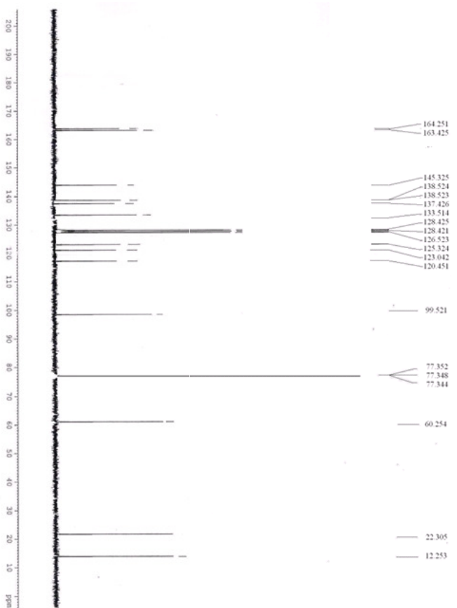
Fig. 4.24 Mass (ESI) spectrum of ethyl 1,4-dihydro-1H-thiochromeno[5,4-c]benzodiazepine-4-carboxylate (8)
