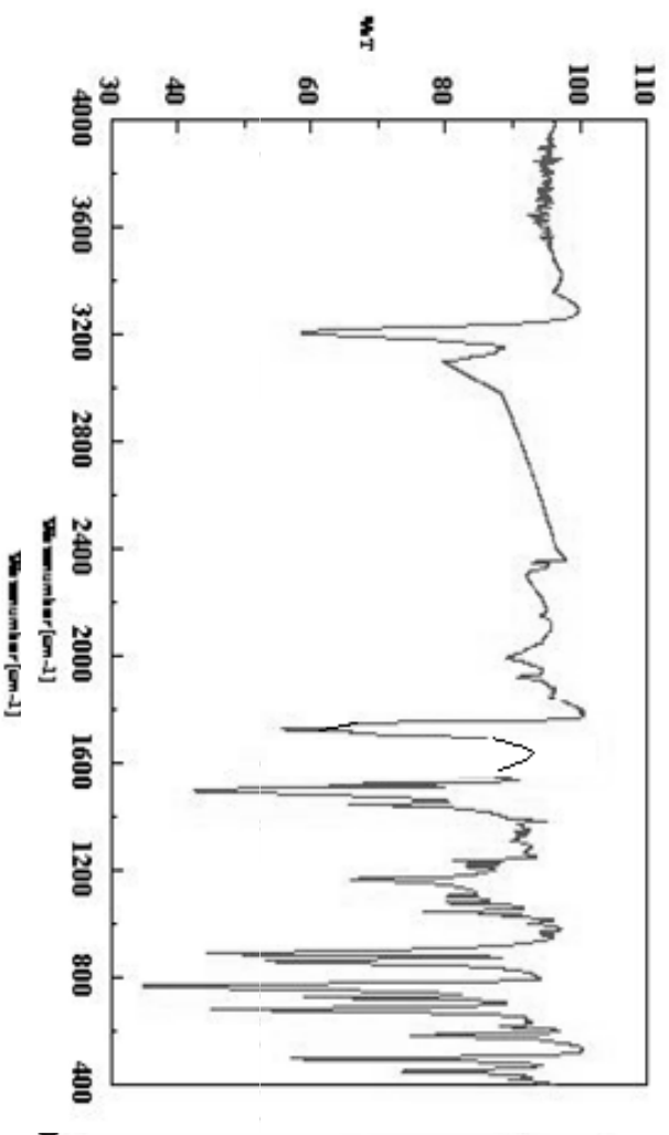
Fig. 4.53 IR (KBr) spectrum of ethyl 2,3-diphenyl-2,3-dihydro-1H-benzothiepine [5,4-c]diazepine-5-carboxylate (18)
