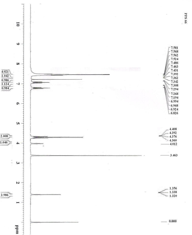
Fig. 4.23 13 C-NMR (CDCl 3 +DMSO-d 6 ) spectrum of ethyl 1,4-dihydro-1H-thiochromenol[5,4-c]benzodiazepine-4-carboxylate (8)
