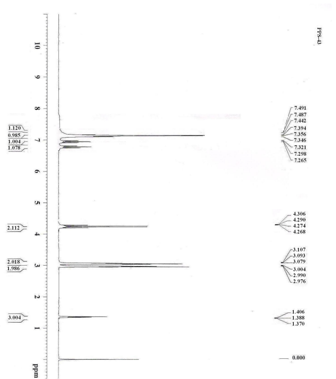
Fig. 4.34 1 H-NMR (CDCl 3 ) spectrum of ethyl 4,5-dihydro-1H-[1]benzothiepinol[5,4-c]pyrazole-3-carboxylate (13)
