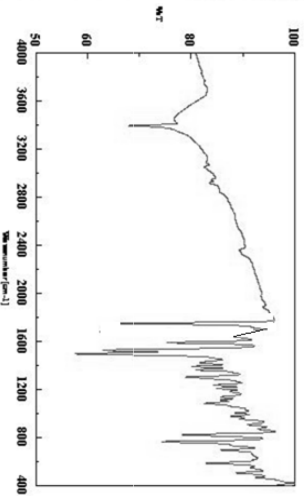
Fig. 4.33 IR (KBr) spectrum of ethyl 4,5-dihydro-1H-[1]benzothiepinol[5,4-c]pyrazole-3-carboxylate (13)
