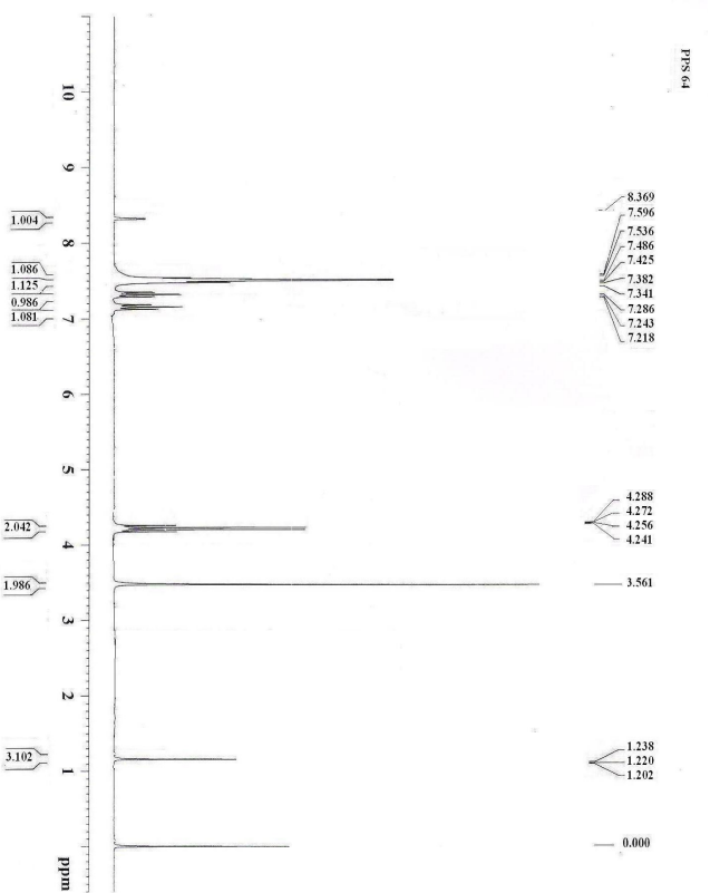
Fig. 4.18 1 H-NMR (CDCl 3 +DMSO-d 6 ) spectrum of ethyl-2,5-dihydro-2-thioxo-1H-thiochromeno[4,3-d]pyrimidine-4-carboxylate (7)
