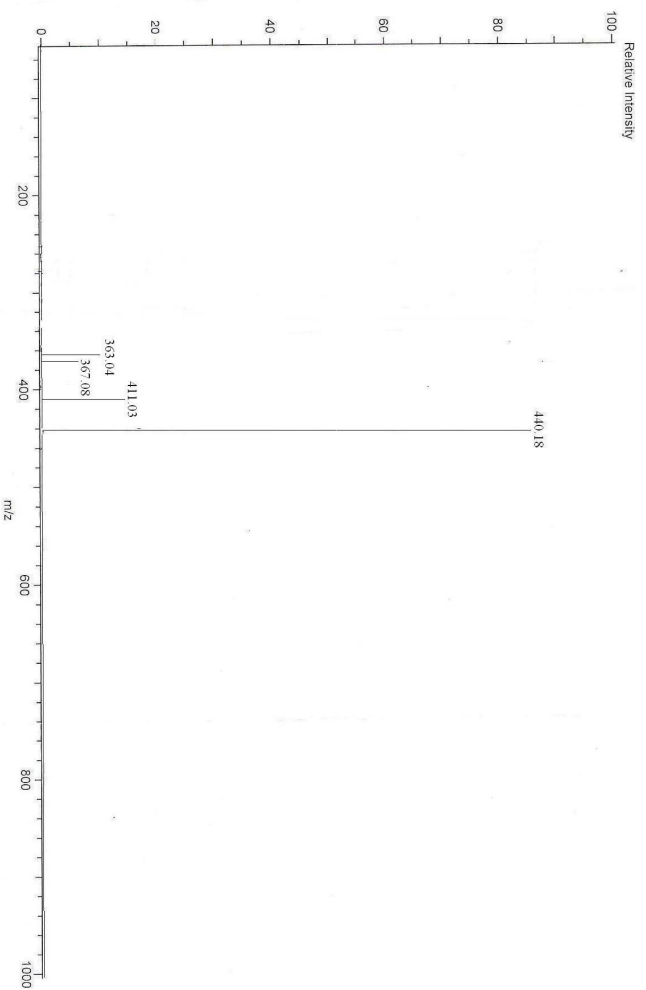
Fig. 4.28 Mass (ESI) spectrum of ethyl 2,3-diphenyl-2,3-dihydro-1H-thiochromeno[5,4-c[diazepine-5-carboxylate (9)
