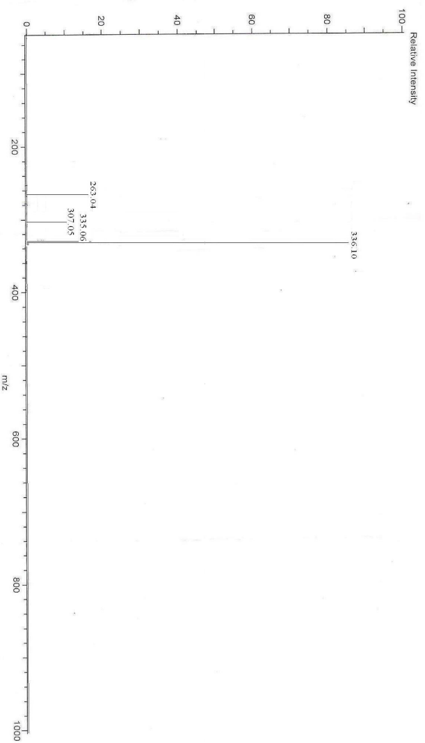
Fig. 4.22 1 H-NMR (CDCl 3 +DMSO-d 6 ) spectrum of ethyl 1,4-dihydro-1H-thiochromeno[5,4-c]benzodiazepine-4-carboxylate (8)
