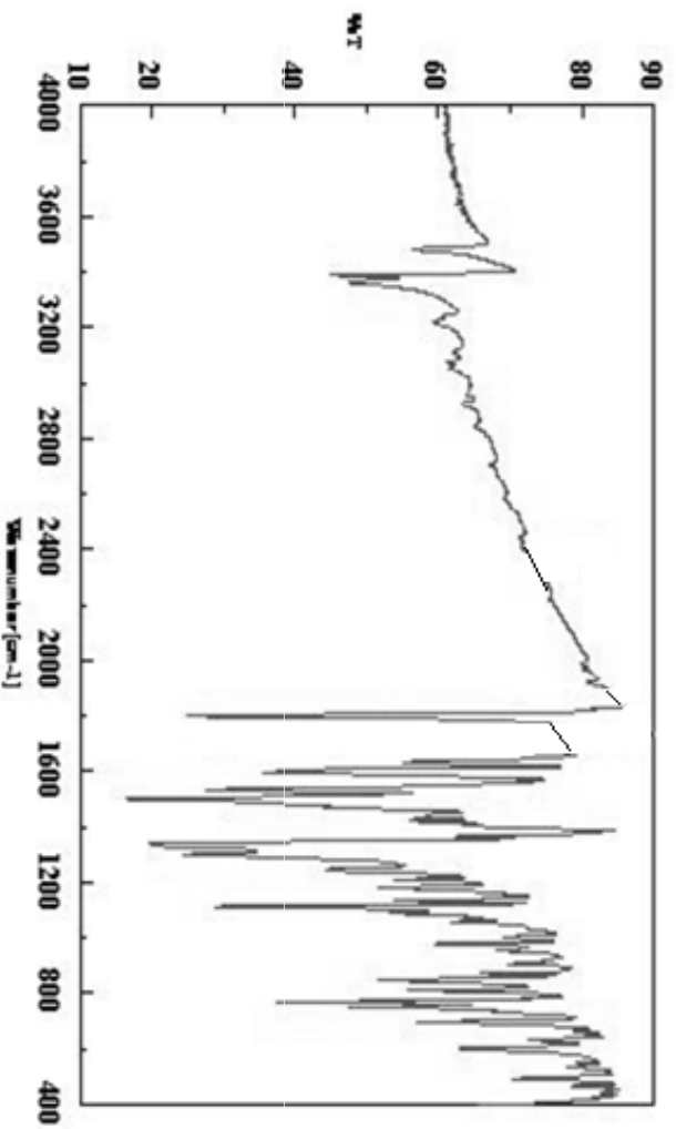
Fig. 4.41 IR (KBr) spectrum of ethyl 2-oxo-1,2,5,6-tetrahydro[1]benzothiepinol[5,4-d]pyrimidine-4-carboxylate (15)
