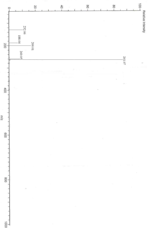
Fig. 4.12 Mass (ESD) spectrum of ethyl 4H-thiochromeno[3,4-d]isoxazole-3-carboxylate (5)
