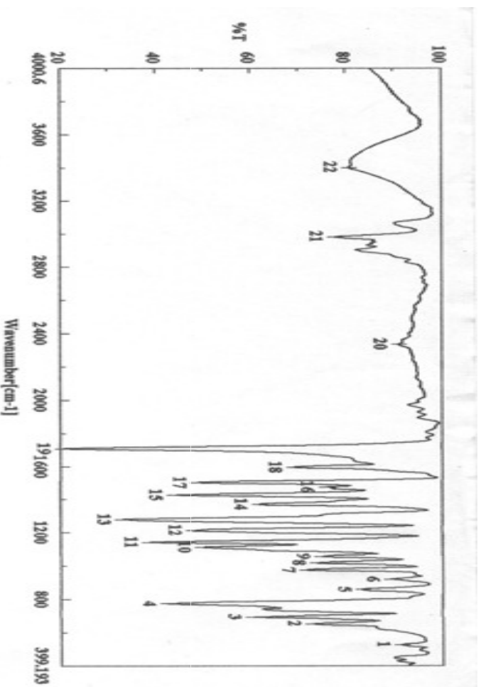
Fig. 4.29 IR (KBr) spectrum of ethyl 1-phenyl-4,5-dihydro-1H-[1]benzothiepinol[5,4-c]pyrazole-3-carboxylate (12)
