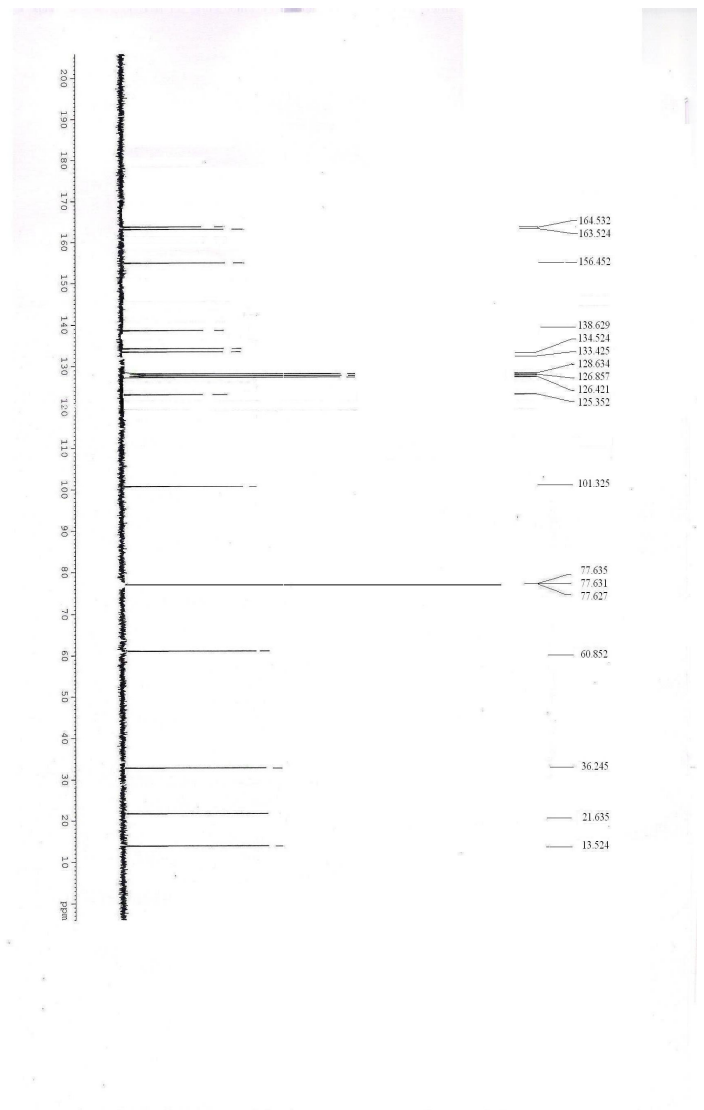
Fig. 4.4313C-NMR (DMSO-d6) spectrum of ethyl-2-oxo-1,2,5,6-tetrahydro[1]benzothiepinol[5,4-tetrahydro]pyrimidine-4-carboxylate (15)
