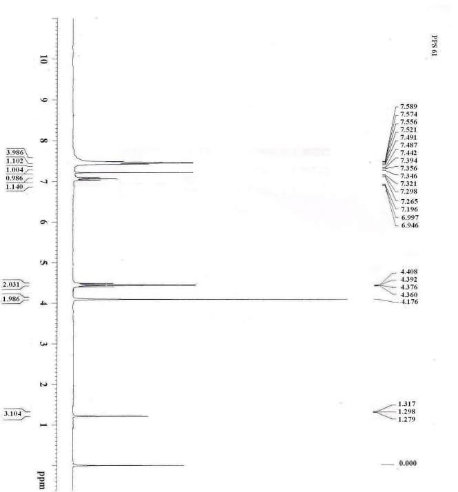
Fig. 4.2 1 H-NMR (CDCl 3 ) spectrum of ethyl-1,4-dihydro-1-phenylthiochromeno[4,3-c]pyrazole-3-carboxylate (3)
