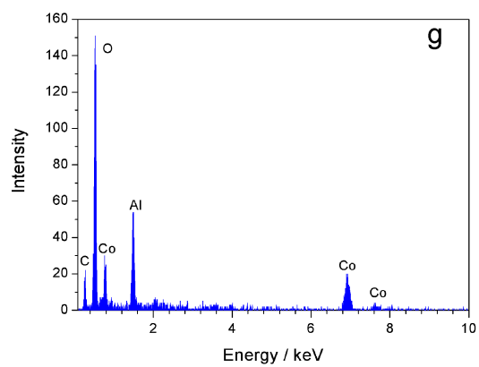
Fig. S1 The electron dispersion X-ray spectra of CoNiAl LDHs with different molar ratio of Co/Ni: (a) 0:1; (b) 1:5; (c) 1:3; (d) 1:1; (e) 3:1; (f) 5:1; (g) 1:0.
