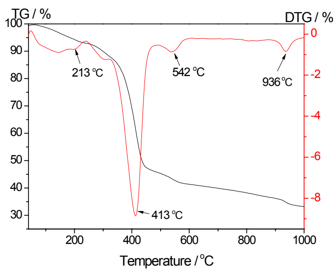
Figure S3 The selected TG-DTG curves of MR-N-Gd-S15 hybrids.
