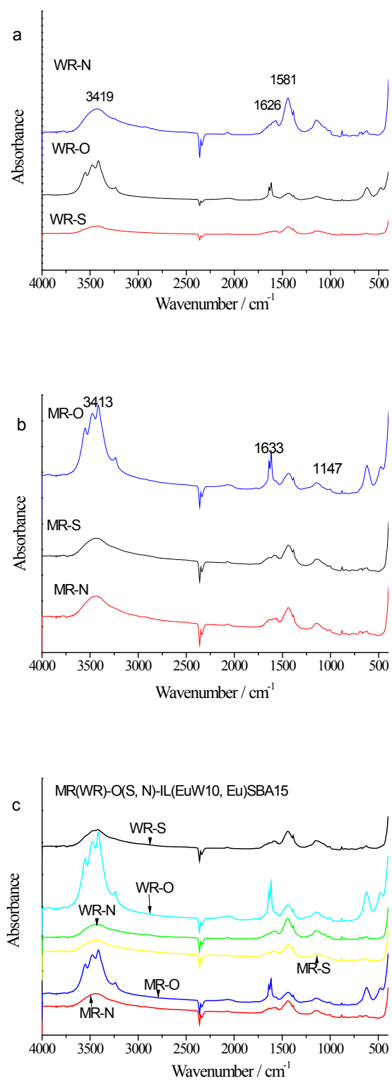
Figure S1 The selected FTIR spectra of WR-O(S, N) (a), MR-O(S, N) (b) and hybrids MR(WR)-O(S, N)-Eu-S15 (c).
