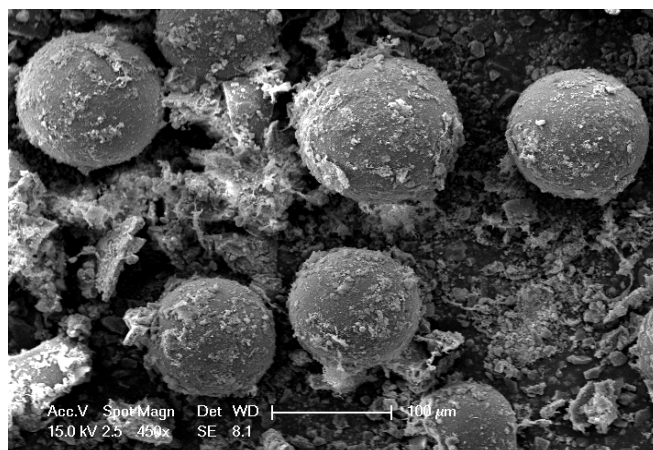
Figure S2 The selected SEM image of MR-O-Gd-S15 hybrids.
