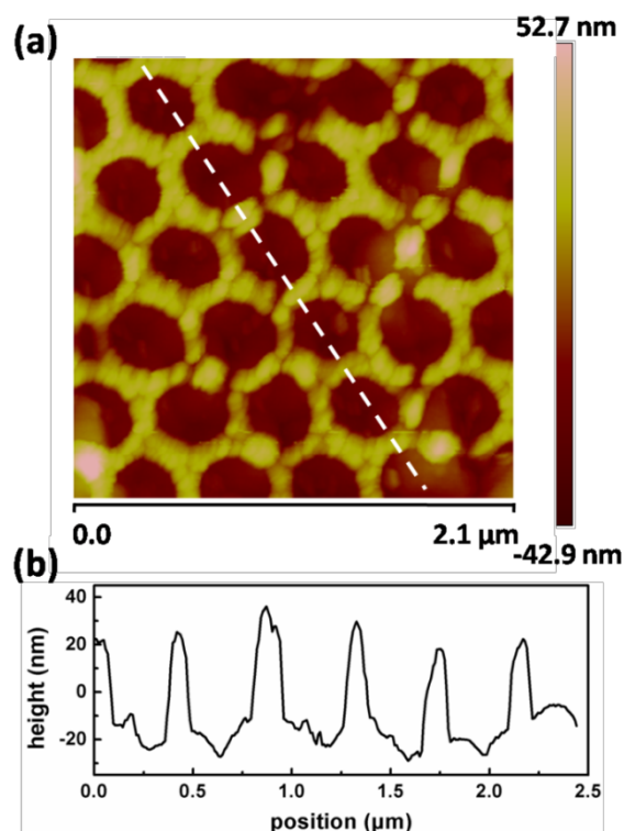
Fig. S2 (a) The 2D AFM image of TiO 2 NBs array, (b) the cross-section of AFM data corresponding to the position of white dot line in Fig. S2(a)
