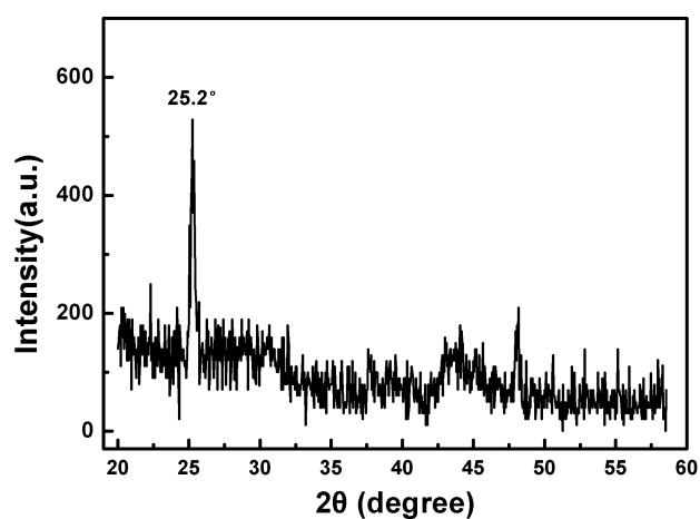
Fig. S1 XRD pattern of the TiO 2 NBs array.
