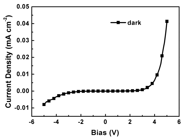
Fig. S3 The J–V characteristics of the device in dark individually (in linear scale).
