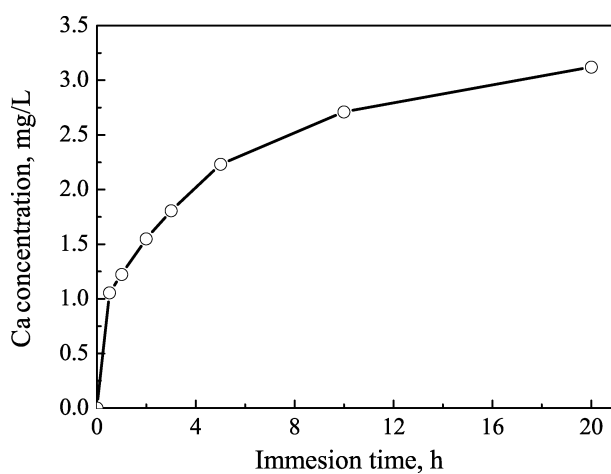
Figure S2. The in vitro Ca release profiles of MEHMs in PBS solution
