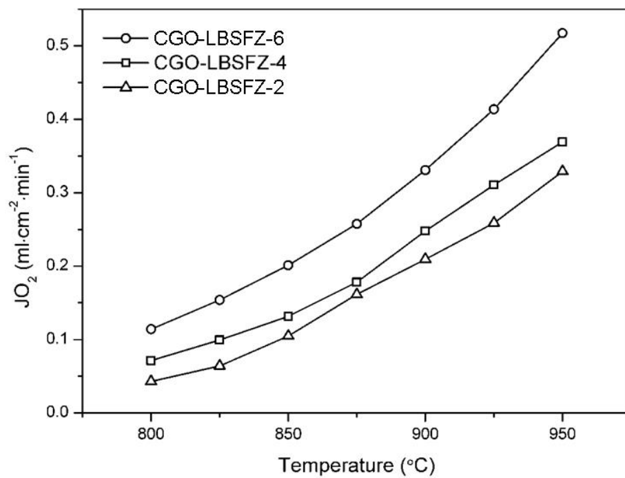
Figure S3: Oxygen permeation fluxes of CGO-LBSFZ membranes as a function of temperature.
