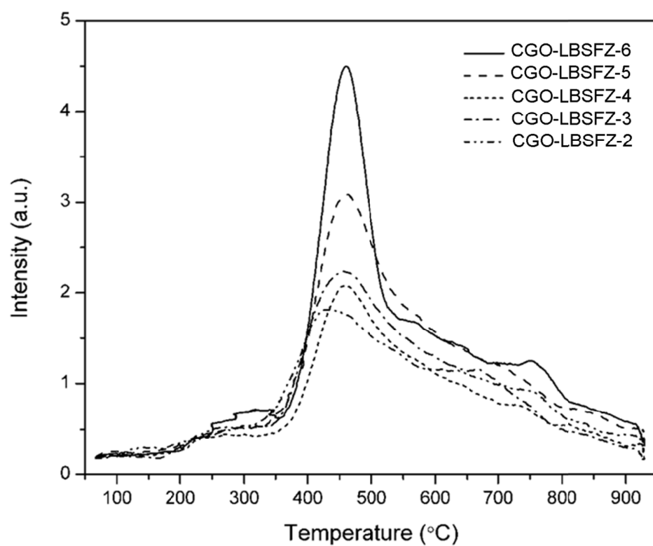
Figure S2: O 2 -TPD profiles of CGO-LBSFZ composites sintered at 1400 °C
