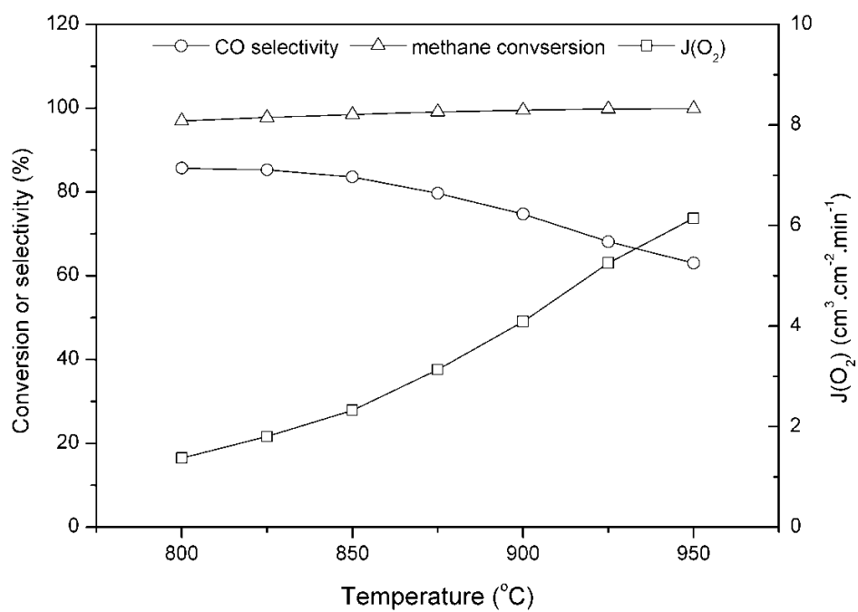
Figure S4: POM reaction of CGO-LBSFZ-6 membrane at 950 °C with 50% CH 4 -He feed gas.
