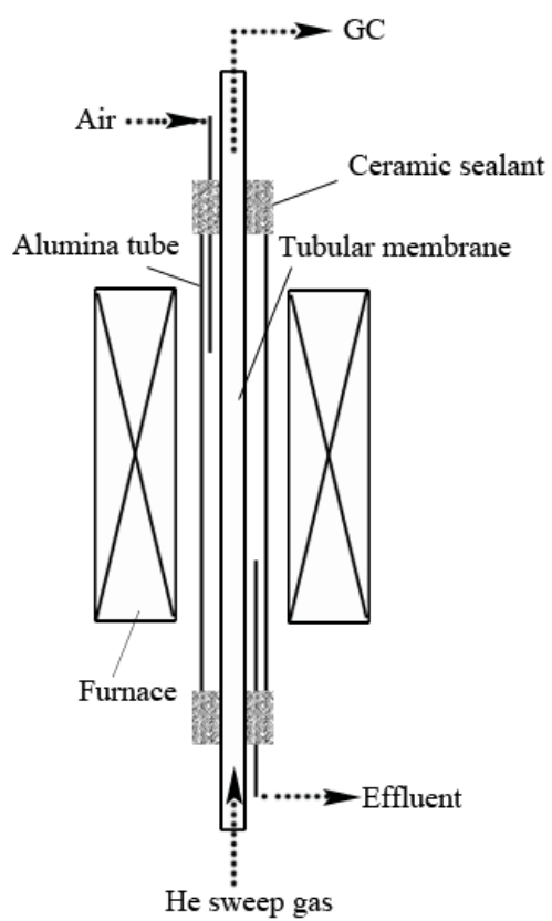
Figure S1: Schematic of oxygen permeation examination of the tubular membrane
