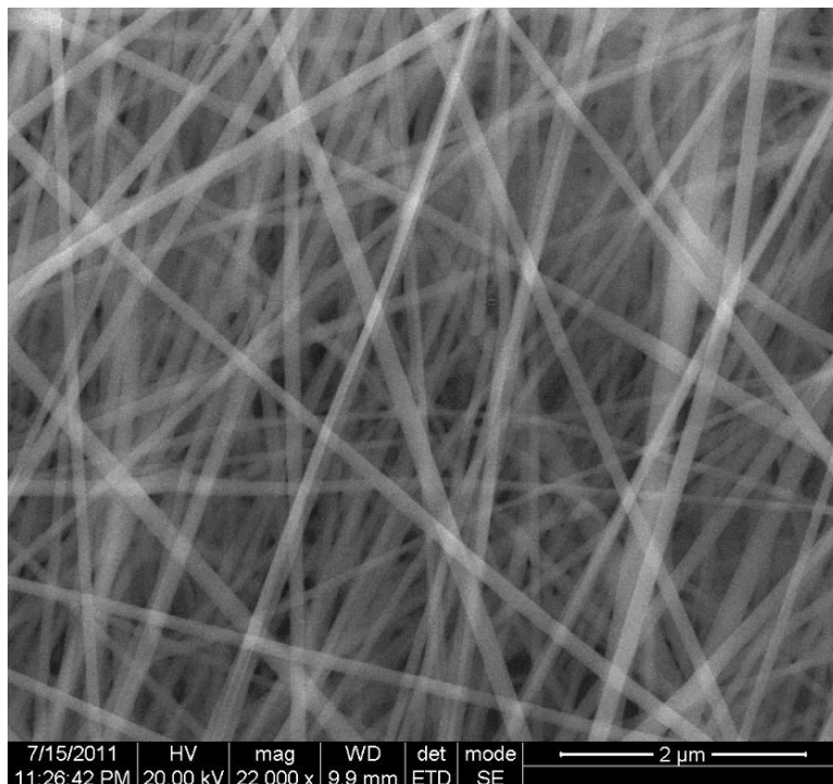
Figure S1 Scanning electron micrographs of PI (neat)
