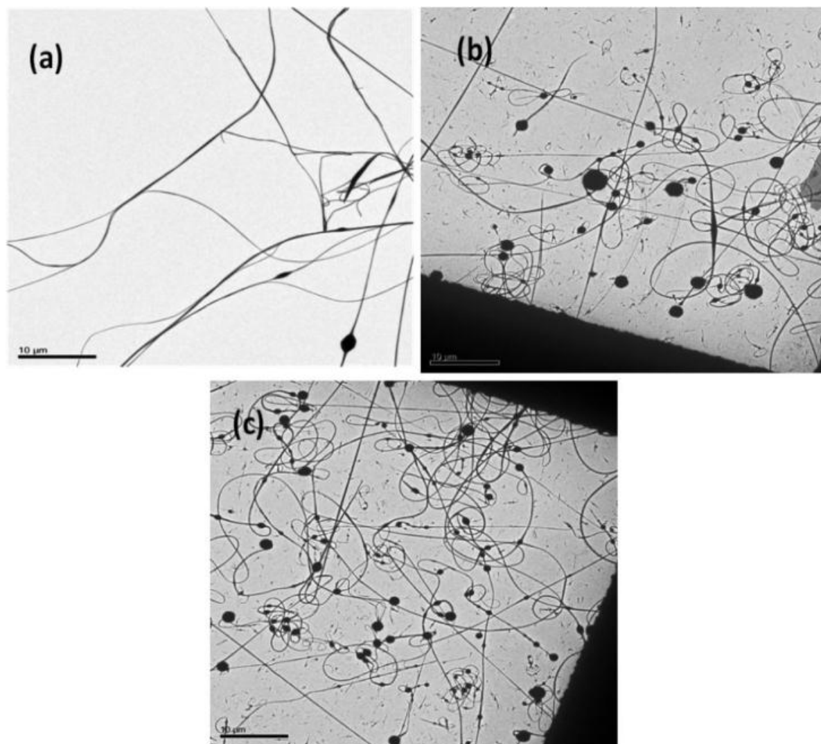
Figure S2 Transmission electron micrographs of GO-PAA with GO contents of 0.1 % (GO) (a), 1% (GO) (b), 2% (GO) (c).
