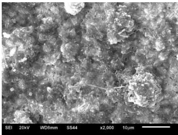
Fig. S1 SDC surface tested by molten carbonate in hydrogen at 700 °C for 24 hours and cleaned by diluted nitric acid
