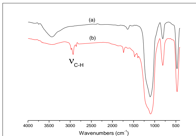
S1. FTIR spectra of SiO 2 particles (a) and SiO 2 -initiator (b)
