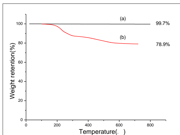
S2. TGA diagram of SiO 2 particles (a) and SiO 2 -initiator (b)
