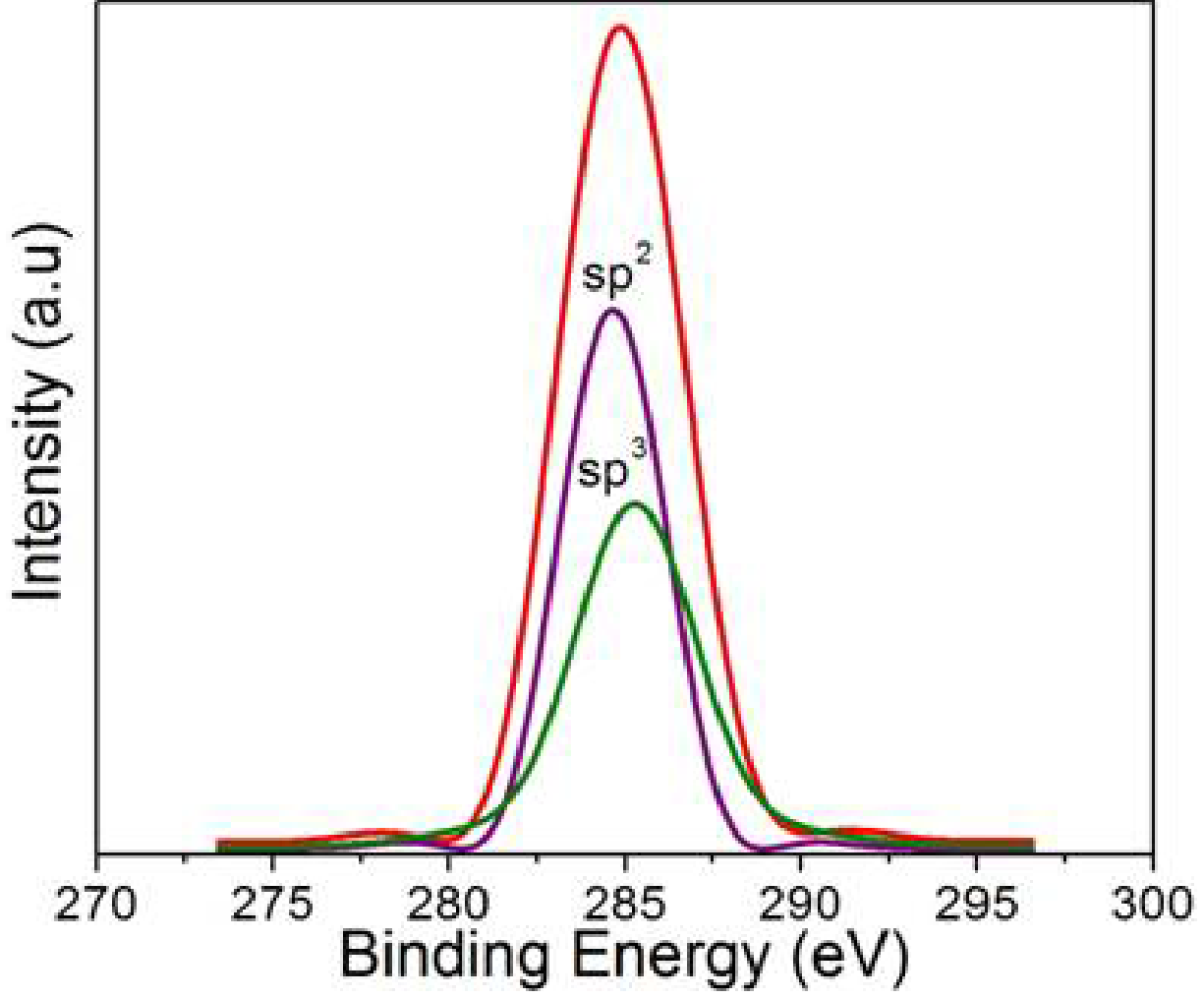
Fig. ESI-2. XPS of NC-2 samples (de-convoluted peaks of carbon)
