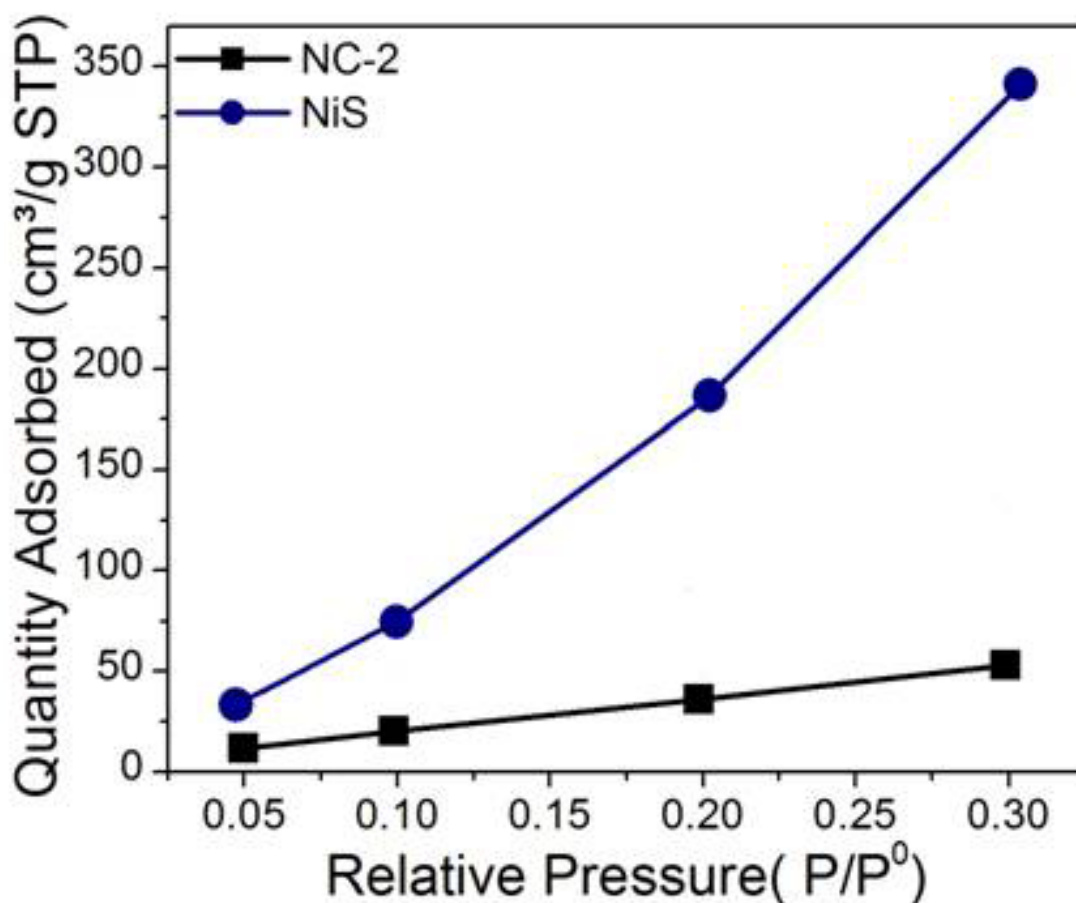
Fig. ESI-1. BET Analysis of NiS and NC-2 samples
