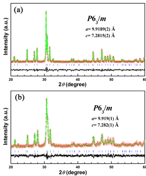
Fig. S1 Rietveld refinement of the XRD patterns of \text{La}_{9.33}\text{Ge}_6\text{O}_{26} powders synthesized by MSS method (a) at 900 °C for 4 h and that synthesized by SSS method (b) at 1100 °C for 4 h, respectively.
