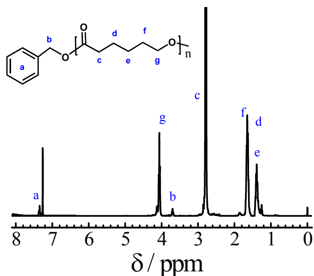
Figure S1. ^1\text{H} NMR spectrum of PCL in \text{CDCl}_3 .
