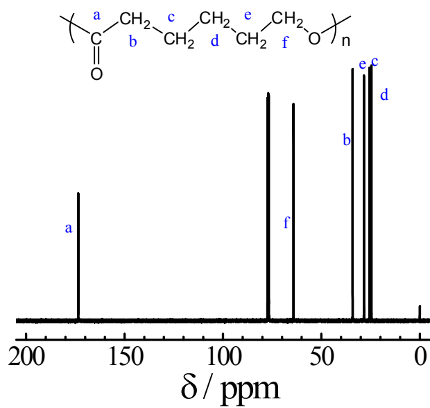
Figure S2. ^{13}C NMR spectrum of PCL in CDCl_3 .
