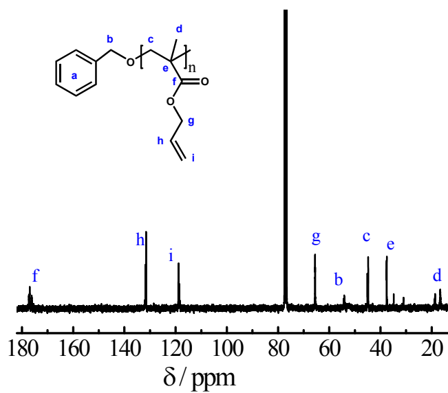
Figure S3. ^{13}C NMR spectrum of PAMA in CDCl_3 .
